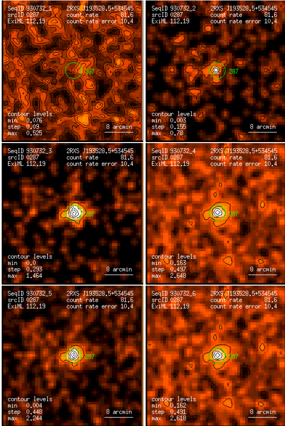
Figure 287: RASS 930732: detection 0287: band rate images, Gaussian filter: (1) PSPC channels 11 – 41, (2) 52 – 90, (3) 91 – 201, (4) 11 – 235, (5) 52 – 201, (6) 11 – 201. Broad band rates in counts/ks. Band rate contour levels in counts/ks/arcmin 2 .
