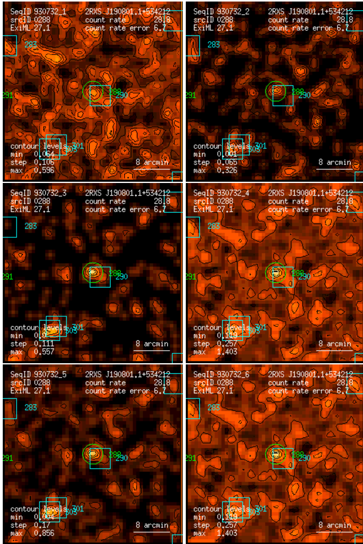
Figure 288: RASS 930732: detection 0288: band rate images, Gaussian filter: (1) PSPC channels 11 – 41, (2) 52 – 90, (3) 91 – 201, (4) 11 – 235, (5) 52 – 201, (6) 11 – 201. Broad band rates in counts/ks. Band rate contour levels in counts/ks/arcmin 2 .
