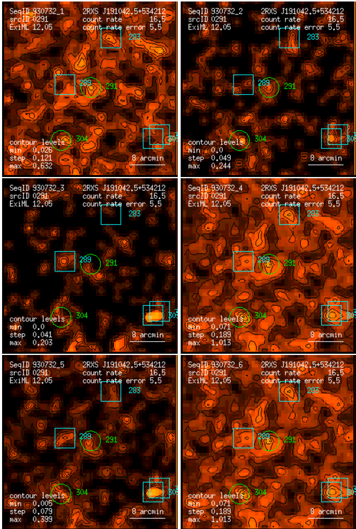
Figure 291: RASS 930732: detection 0291: band rate images, Gaussian filter: (1) PSPC channels 11 – 41, (2) 52 – 90, (3) 91 – 201, (4) 11 – 235, (5) 52 – 201, (6) 11 – 201. Broad band rates in counts/ks. Band rate contour levels in counts/ks/arcmin 2 .
