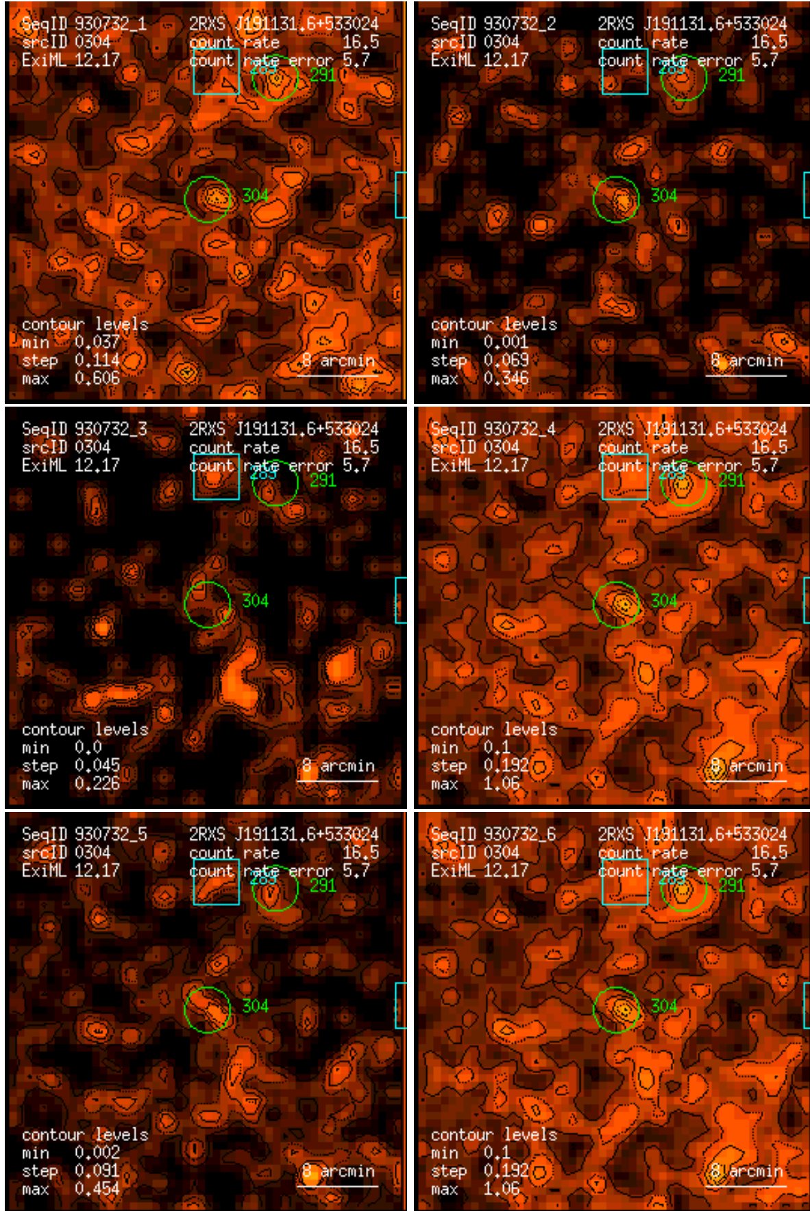
Figure 304: RASS 930732: detection 0304: band rate images, Gaussian filter: (1) PSPC channels 11 – 41, (2) 52 – 90, (3) 91 – 201, (4) 11 – 235, (5) 52 – 201, (6) 11 – 201. Broad band rates in counts/ks. Band rate contour levels in counts/ks/arcmin 2 .
