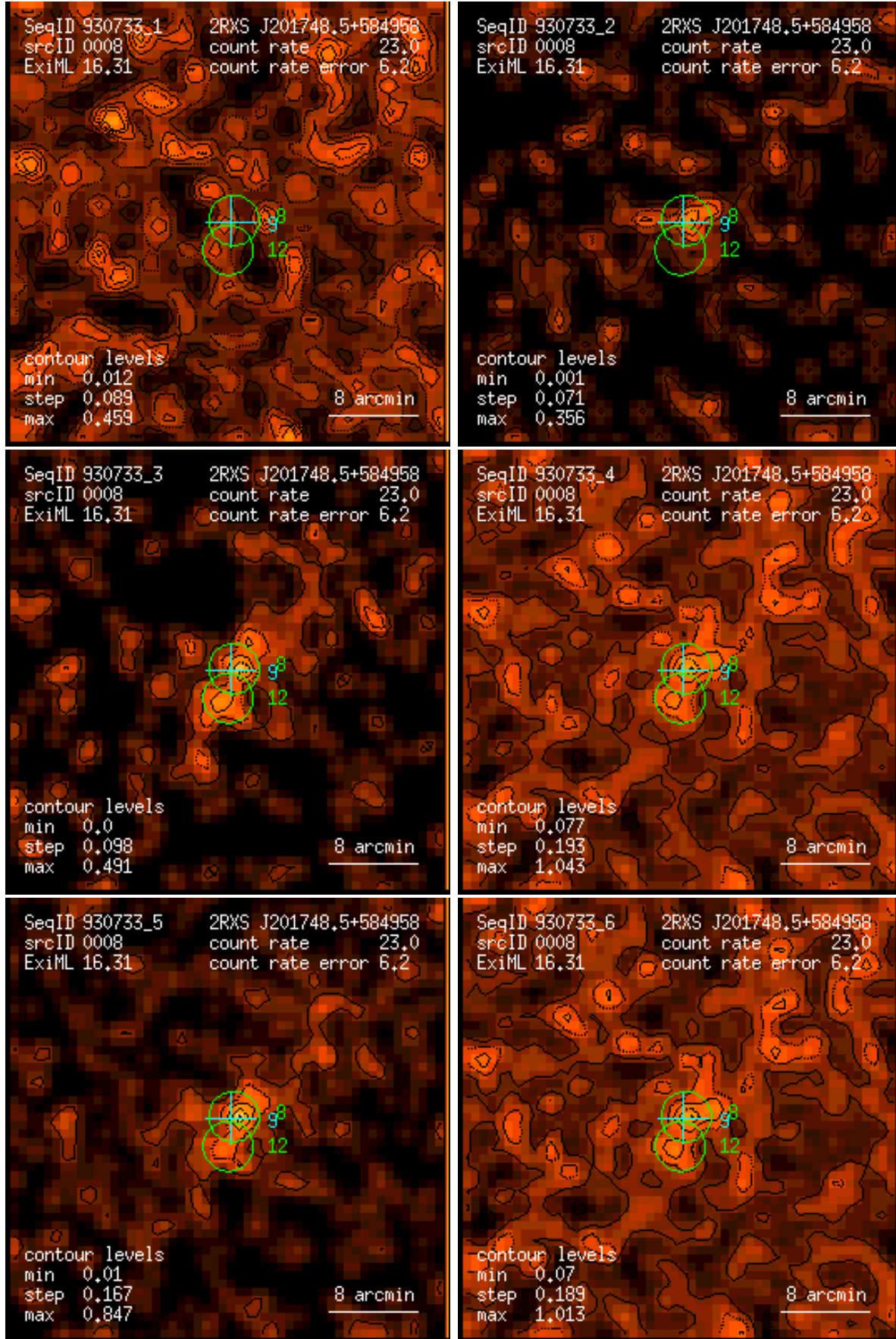
Figure 8: RASS 930733: detection 0008: band rate images, Gaussian filter: (1) PSPC channels 11 – 41, (2) 52 – 90, (3) 91 – 201, (4) 11 – 235, (5) 52 – 201, (6) 11 – 201. Broad band rates in counts/ks. Band rate contour levels in counts/ks/arcmin 2 .
