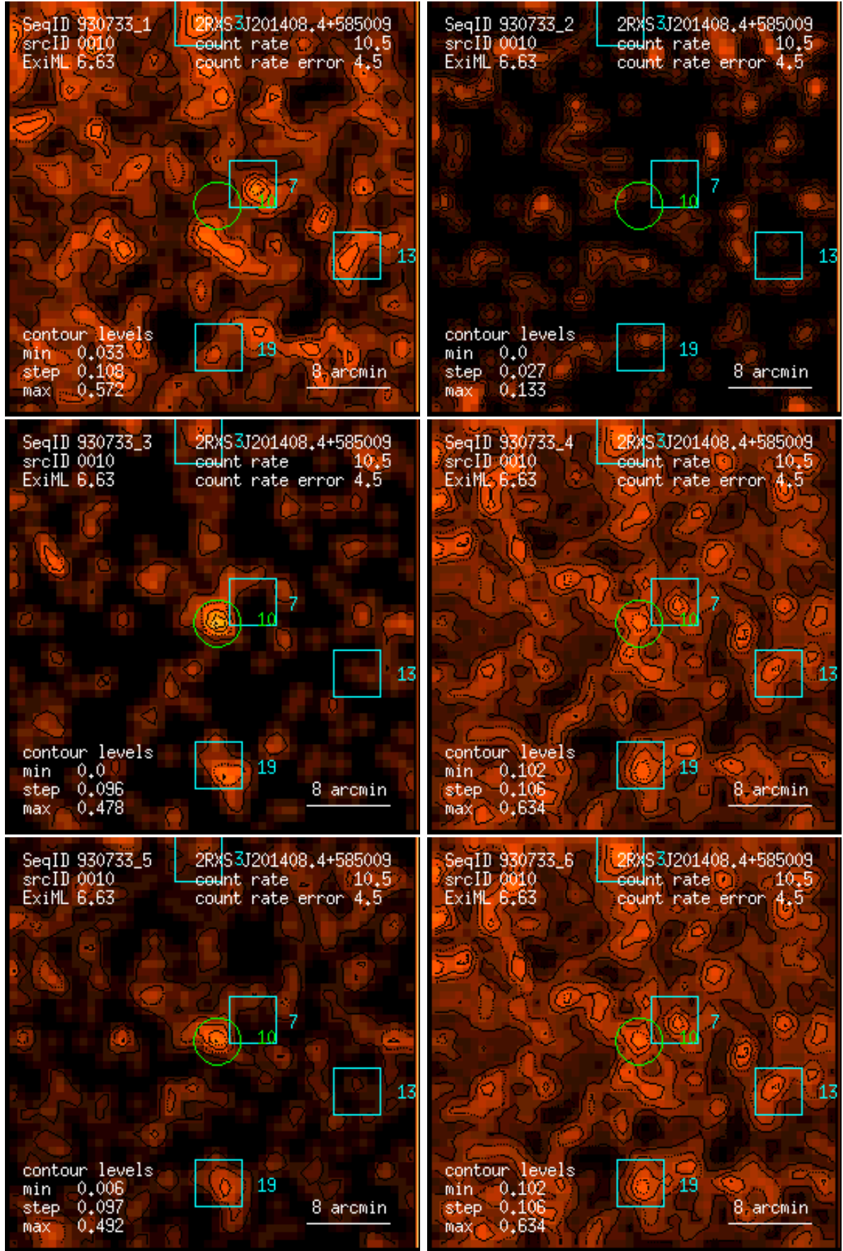
Figure 10: RASS 930733: detection 0010: band rate images, Gaussian filter: (1) PSPC channels 11 – 41, (2) 52 – 90, (3) 91 – 201, (4) 11 – 235, (5) 52 – 201, (6) 11 – 201. Broad band rates in counts/ks. Band rate contour levels in counts/ks/arcmin 2 .
