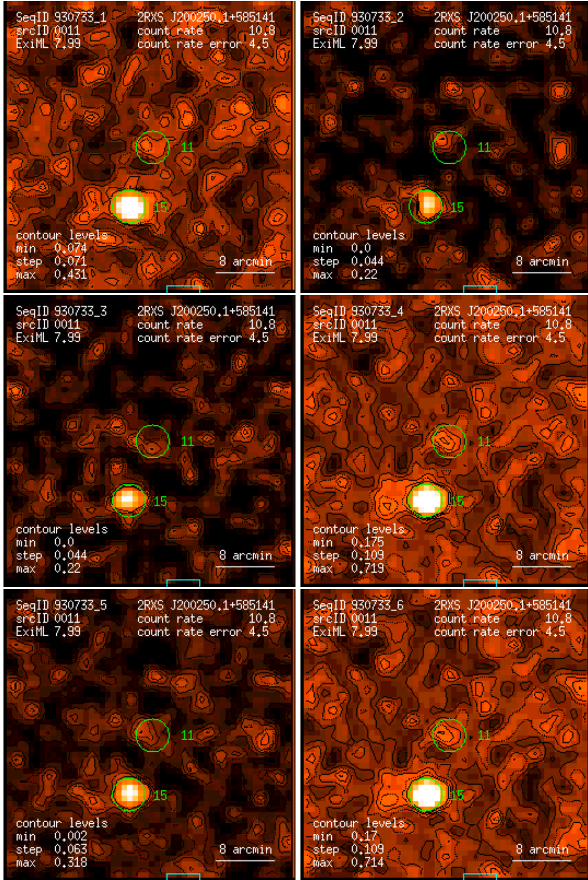
Figure 11: RASS 930733: detection 0011: band rate images, Gaussian filter: (1) PSPC channels 11 – 41, (2) 52 – 90, (3) 91 – 201, (4) 11 – 235, (5) 52 – 201, (6) 11 – 201. Broad band rates in counts/ks. Band rate contour levels in counts/ks/arcmin 2 .
