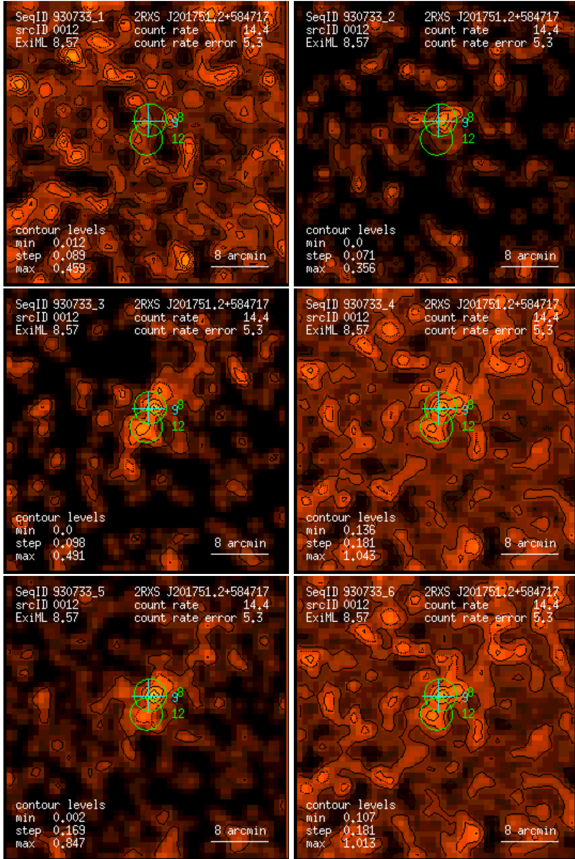
Figure 12: RASS 930733: detection 0012: band rate images, Gaussian filter: (1) PSPC channels 11 – 41, (2) 52 – 90, (3) 91 – 201, (4) 11 – 235, (5) 52 – 201, (6) 11 – 201. Broad band rates in counts/ks. Band rate contour levels in counts/ks/arcmin 2 .
