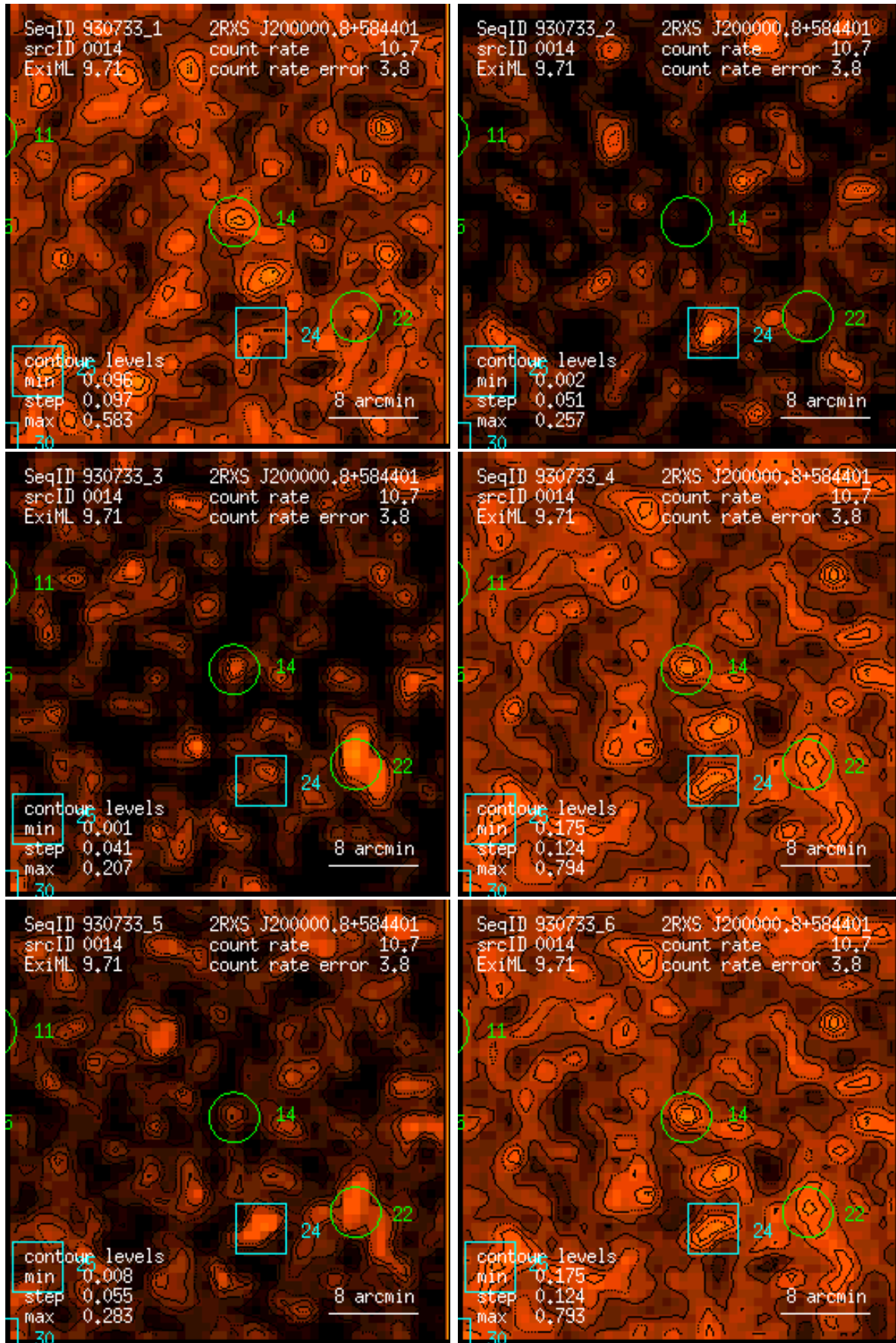
Figure 14: RASS 930733: detection 0014: band rate images, Gaussian filter: (1) PSPC channels 11 – 41, (2) 52 – 90, (3) 91 – 201, (4) 11 – 235, (5) 52 – 201, (6) 11 – 201. Broad band rates in counts/ks. Band rate contour levels in counts/ks/arcmin 2 .
