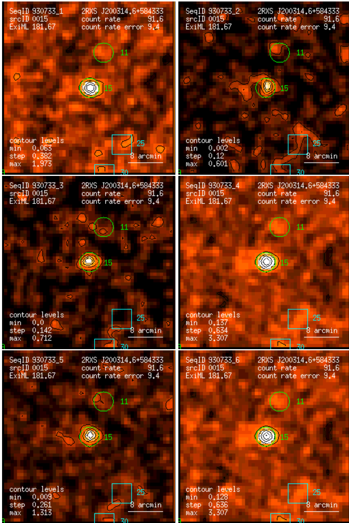
Figure 15: RASS 930733: detection 0015: band rate images, Gaussian filter: (1) PSPC channels 11 – 41, (2) 52 – 90, (3) 91 – 201, (4) 11 – 235, (5) 52 – 201, (6) 11 – 201. Broad band rates in counts/ks. Band rate contour levels in counts/ks/arcmin 2 .
