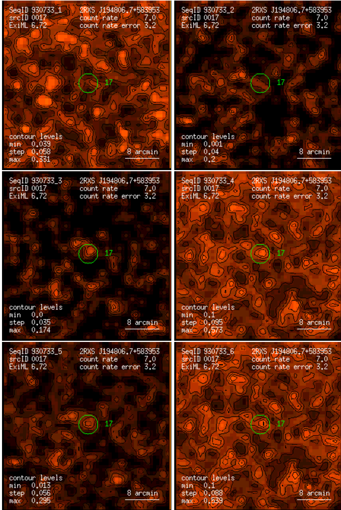
Figure 17: RASS 930733: detection 0017: band rate images, Gaussian filter: (1) PSPC channels 11 – 41, (2) 52 – 90, (3) 91 – 201, (4) 11 – 235, (5) 52 – 201, (6) 11 – 201. Broad band rates in counts/ks. Band rate contour levels in counts/ks/arcmin 2 .
