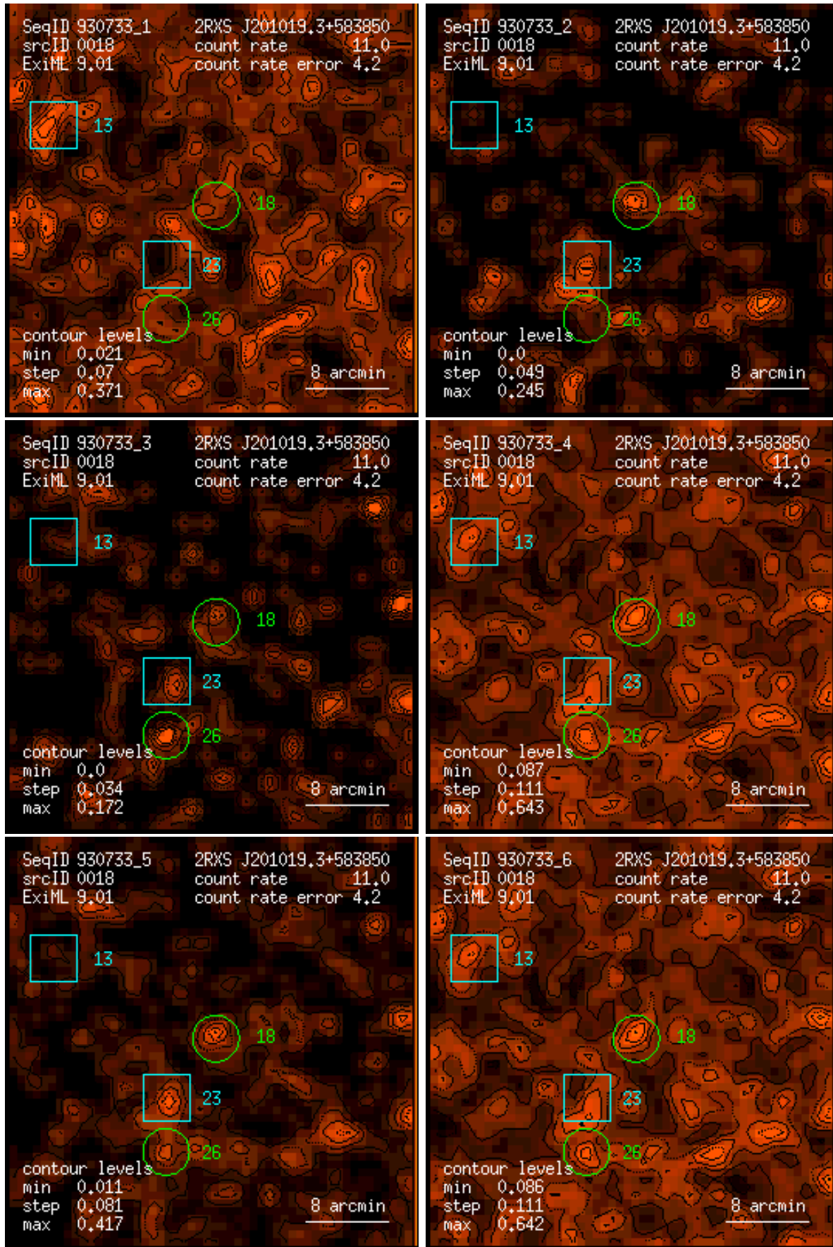
Figure 18: RASS 930733: detection 0018: band rate images, Gaussian filter: (1) PSPC channels 11 – 41, (2) 52 – 90, (3) 91 – 201, (4) 11 – 235, (5) 52 – 201, (6) 11 – 201. Broad band rates in counts/ks. Band rate contour levels in counts/ks/arcmin 2 .
