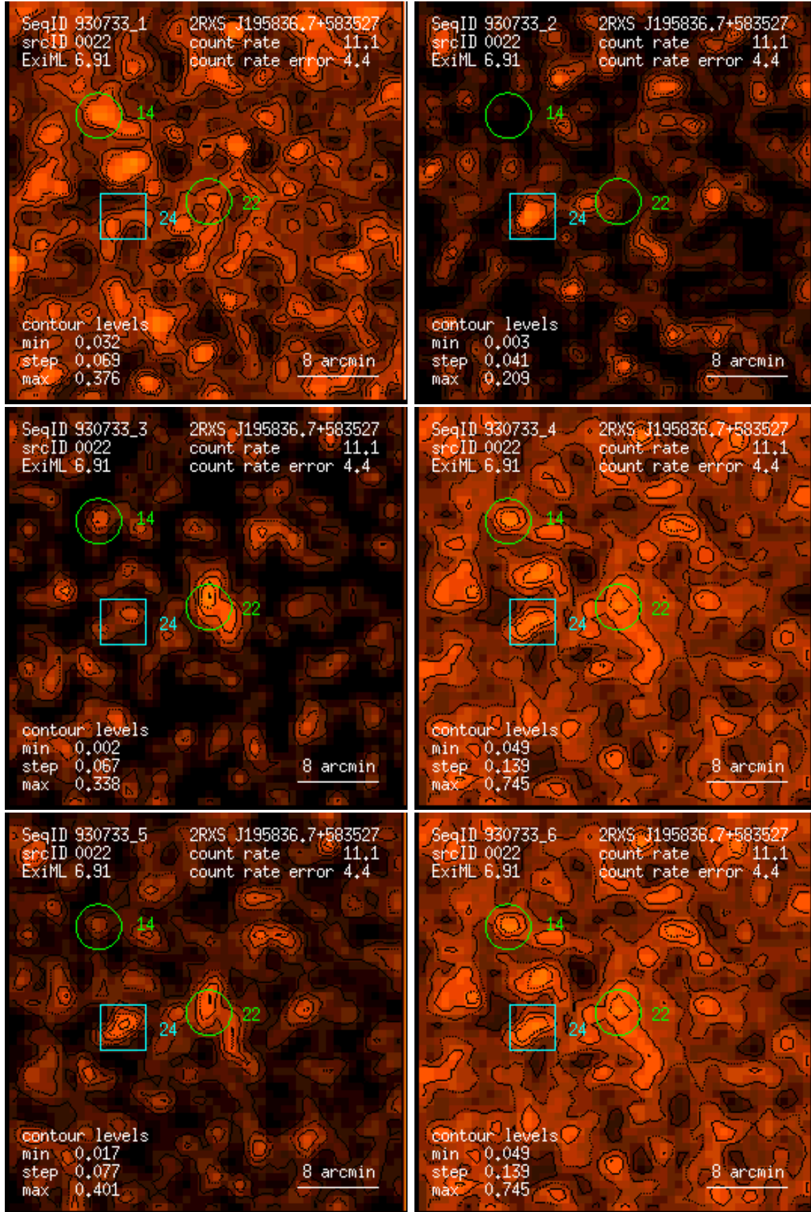
Figure 22: RASS 930733: detection 0022: band rate images, Gaussian filter: (1) PSPC channels 11 – 41, (2) 52 – 90, (3) 91 – 201, (4) 11 – 235, (5) 52 – 201, (6) 11 – 201. Broad band rates in counts/ks. Band rate contour levels in counts/ks/arcmin 2 .
