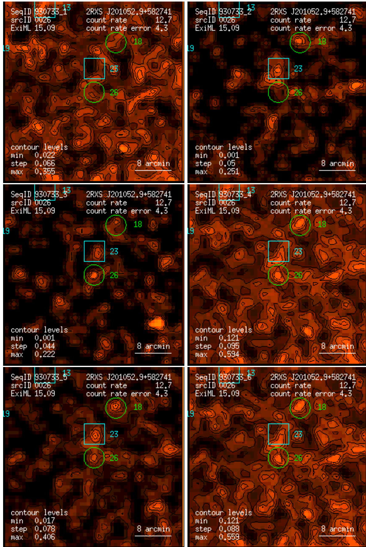
Figure 26: RASS 930733: detection 0026: band rate images, Gaussian filter: (1) PSPC channels 11 – 41, (2) 52 – 90, (3) 91 – 201, (4) 11 – 235, (5) 52 – 201, (6) 11 – 201. Broad band rates in counts/ks. Band rate contour levels in counts/ks/arcmin 2 .
