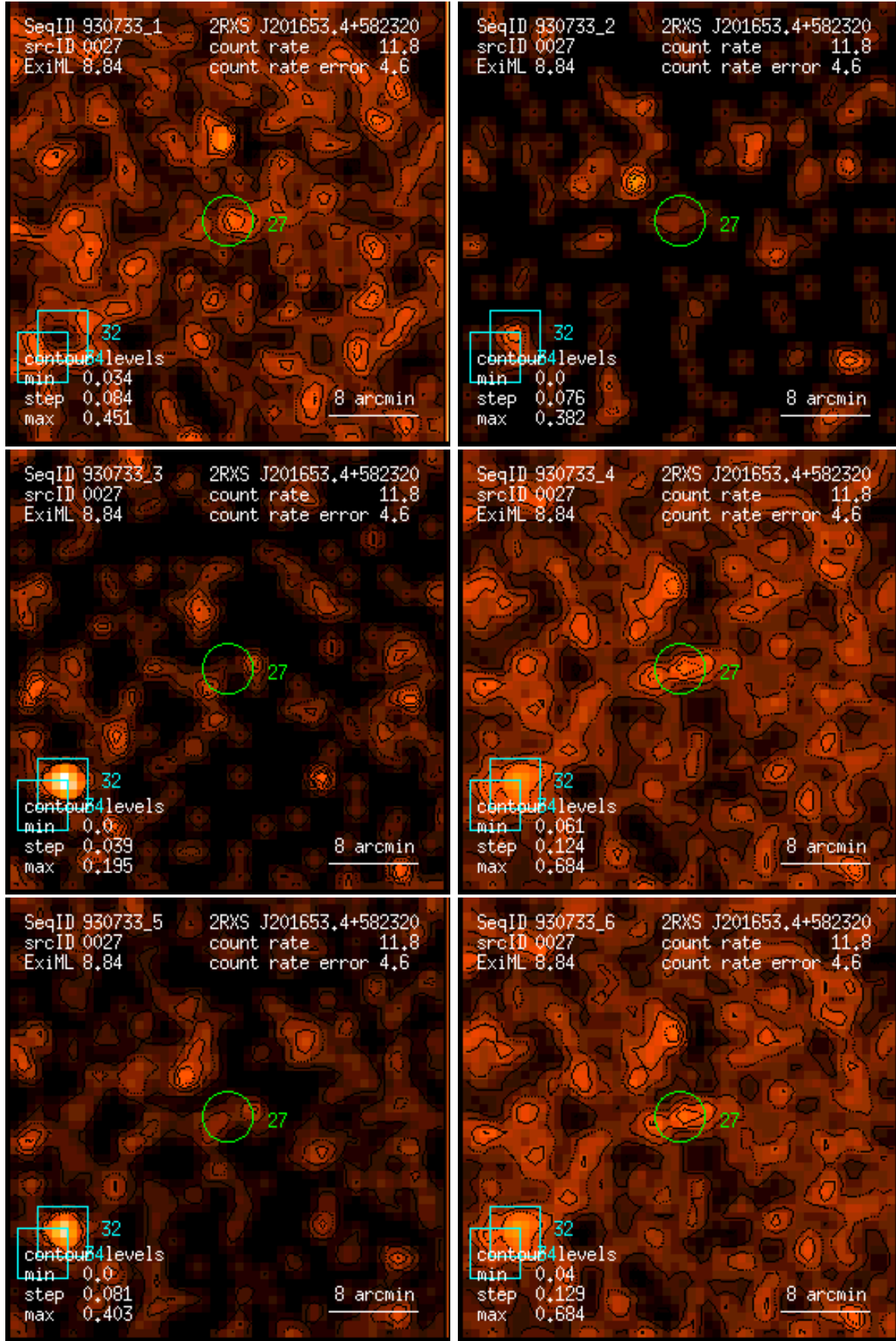
Figure 27: RASS 930733: detection 0027: band rate images, Gaussian filter: (1) PSPC channels 11 – 41, (2) 52 – 90, (3) 91 – 201, (4) 11 – 235, (5) 52 – 201, (6) 11 – 201. Broad band rates in counts/ks. Band rate contour levels in counts/ks/arcmin 2 .
