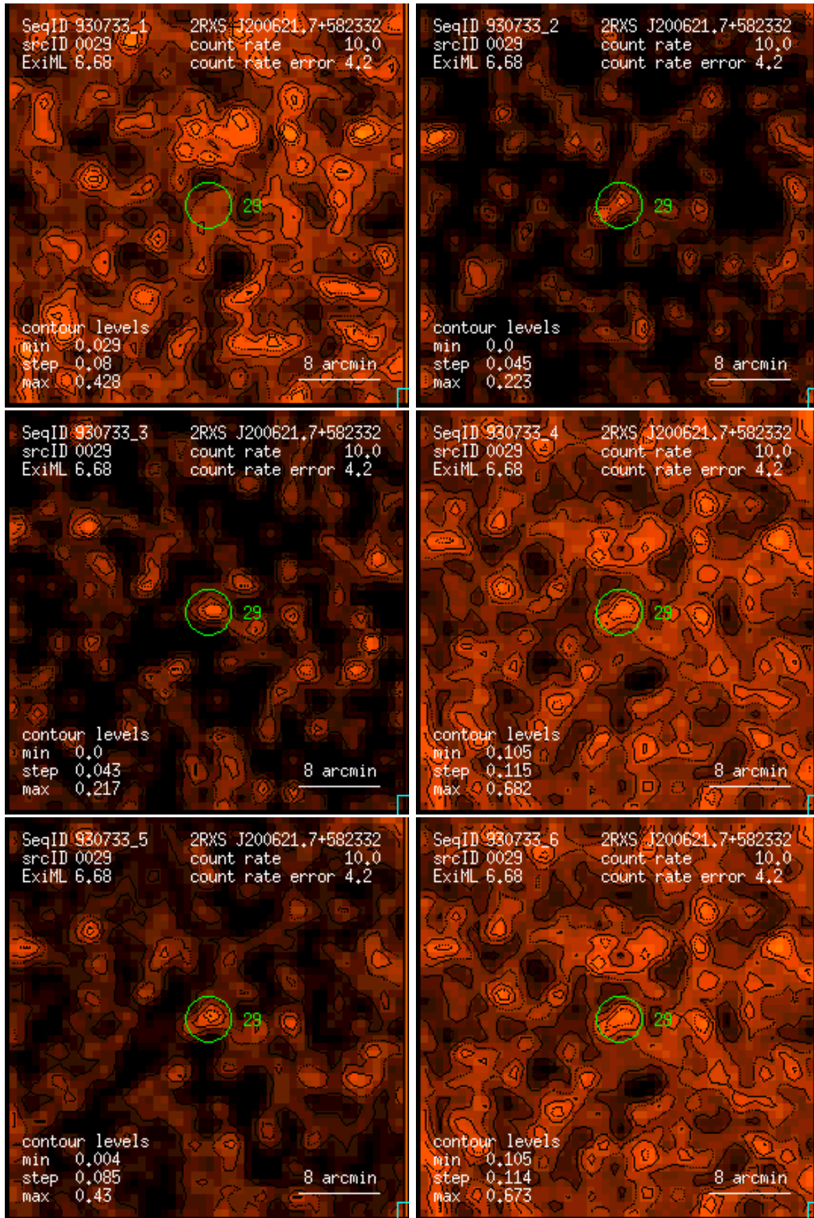
Figure 29: RASS 930733: detection 0029: band rate images, Gaussian filter: (1) PSPC channels 11 – 41, (2) 52 – 90, (3) 91 – 201, (4) 11 – 235, (5) 52 – 201, (6) 11 – 201. Broad band rates in counts/ks. Band rate contour levels in counts/ks/arcmin 2 .
