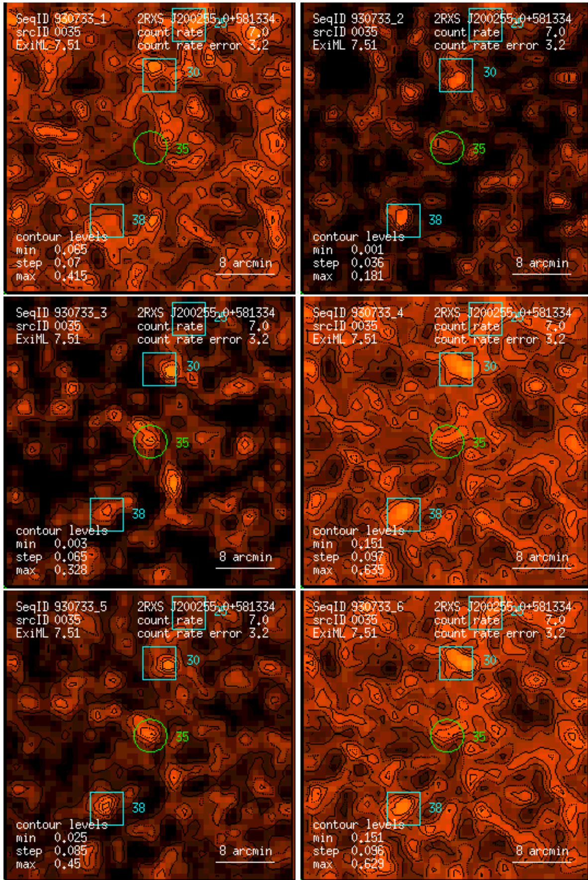
Figure 35: RASS 930733: detection 0035: band rate images, Gaussian filter: (1) PSPC channels 11 – 41, (2) 52 – 90, (3) 91 – 201, (4) 11 – 235, (5) 52 – 201, (6) 11 – 201. Broad band rates in counts/ks. Band rate contour levels in counts/ks/arcmin 2 .
