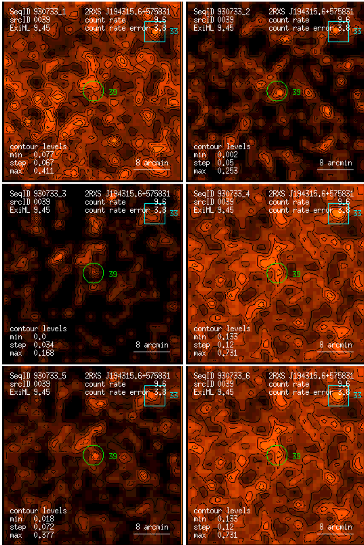
Figure 39: RASS 930733: detection 0039: band rate images, Gaussian filter: (1) PSPC channels 11 – 41, (2) 52 – 90, (3) 91 – 201, (4) 11 – 235, (5) 52 – 201, (6) 11 – 201. Broad band rates in counts/ks. Band rate contour levels in counts/ks/arcmin 2 .
