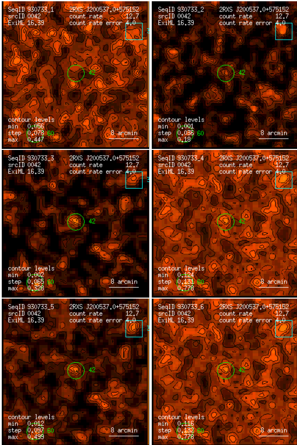
Figure 42: RASS 930733: detection 0042: band rate images, Gaussian filter: (1) PSPC channels 11 – 41, (2) 52 – 90, (3) 91 – 201, (4) 11 – 235, (5) 52 – 201, (6) 11 – 201. Broad band rates in counts/ks. Band rate contour levels in counts/ks/arcmin 2 .
