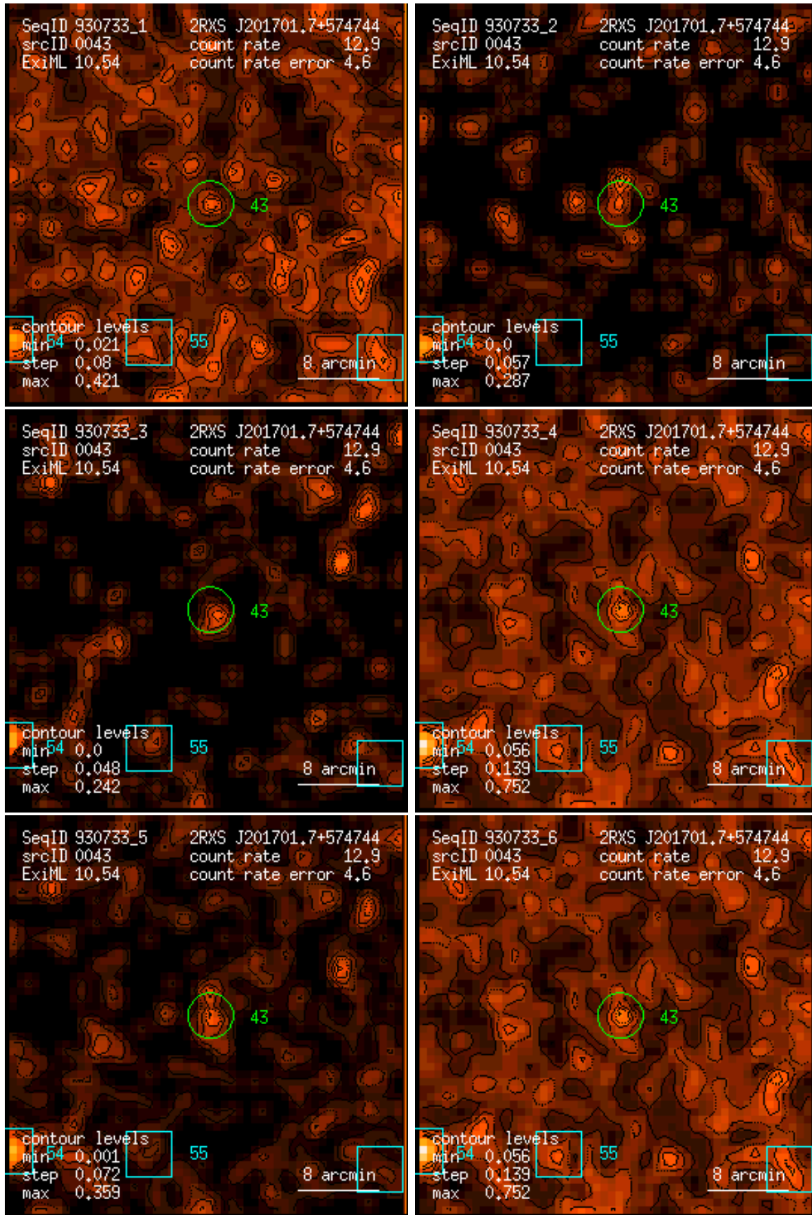
Figure 43: RASS 930733: detection 0043: band rate images, Gaussian filter: (1) PSPC channels 11 – 41, (2) 52 – 90, (3) 91 – 201, (4) 11 – 235, (5) 52 – 201, (6) 11 – 201. Broad band rates in counts/ks. Band rate contour levels in counts/ks/arcmin 2 .
