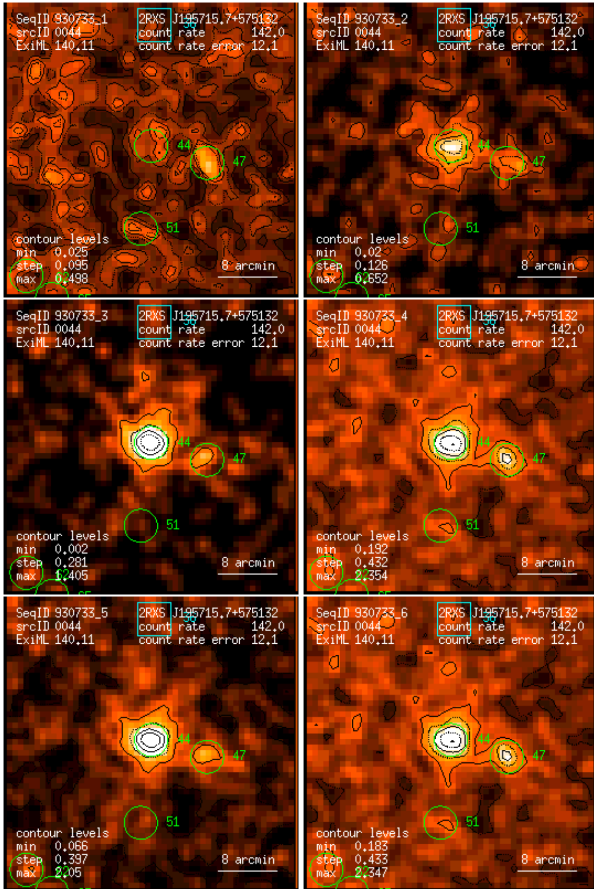
Figure 44: RASS 930733: detection 0044: band rate images, Gaussian filter: (1) PSPC channels 11 – 41, (2) 52 – 90, (3) 91 – 201, (4) 11 – 235, (5) 52 – 201, (6) 11 – 201. Broad band rates in counts/ks. Band rate contour levels in counts/ks/arcmin 2 .
