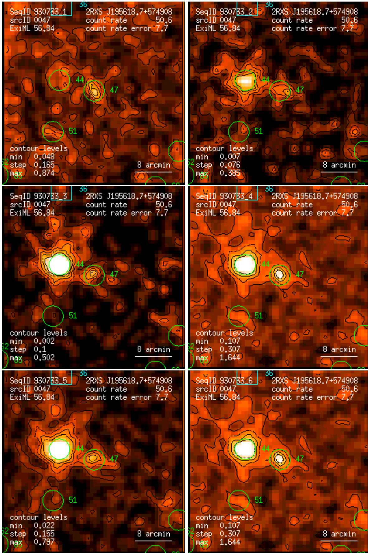
Figure 47: RASS 930733: detection 0047: band rate images, Gaussian filter: (1) PSPC channels 11 – 41, (2) 52 – 90, (3) 91 – 201, (4) 11 – 235, (5) 52 – 201, (6) 11 – 201. Broad band rates in counts/ks. Band rate contour levels in counts/ks/arcmin 2 .
