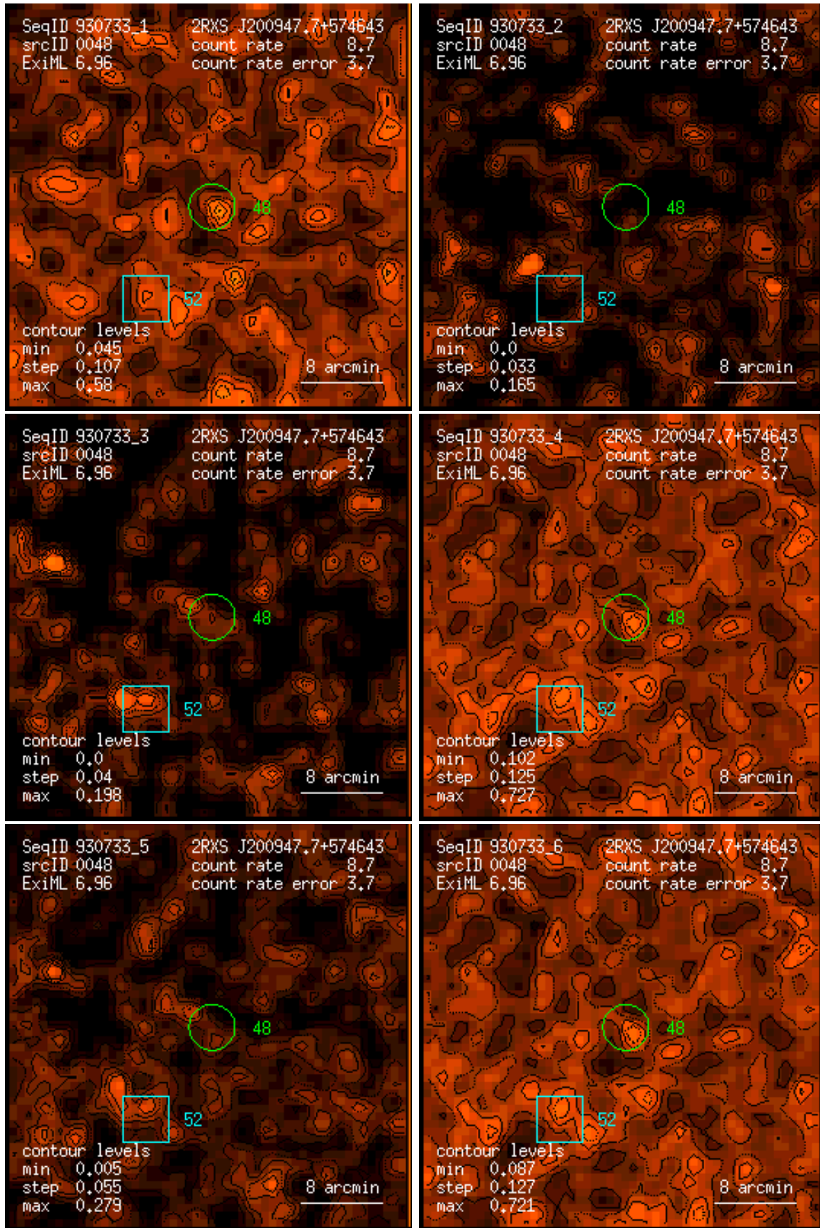
Figure 48: RASS 930733: detection 0048: band rate images, Gaussian filter: (1) PSPC channels 11 – 41, (2) 52 – 90, (3) 91 – 201, (4) 11 – 235, (5) 52 – 201, (6) 11 – 201. Broad band rates in counts/ks. Band rate contour levels in counts/ks/arcmin 2 .
