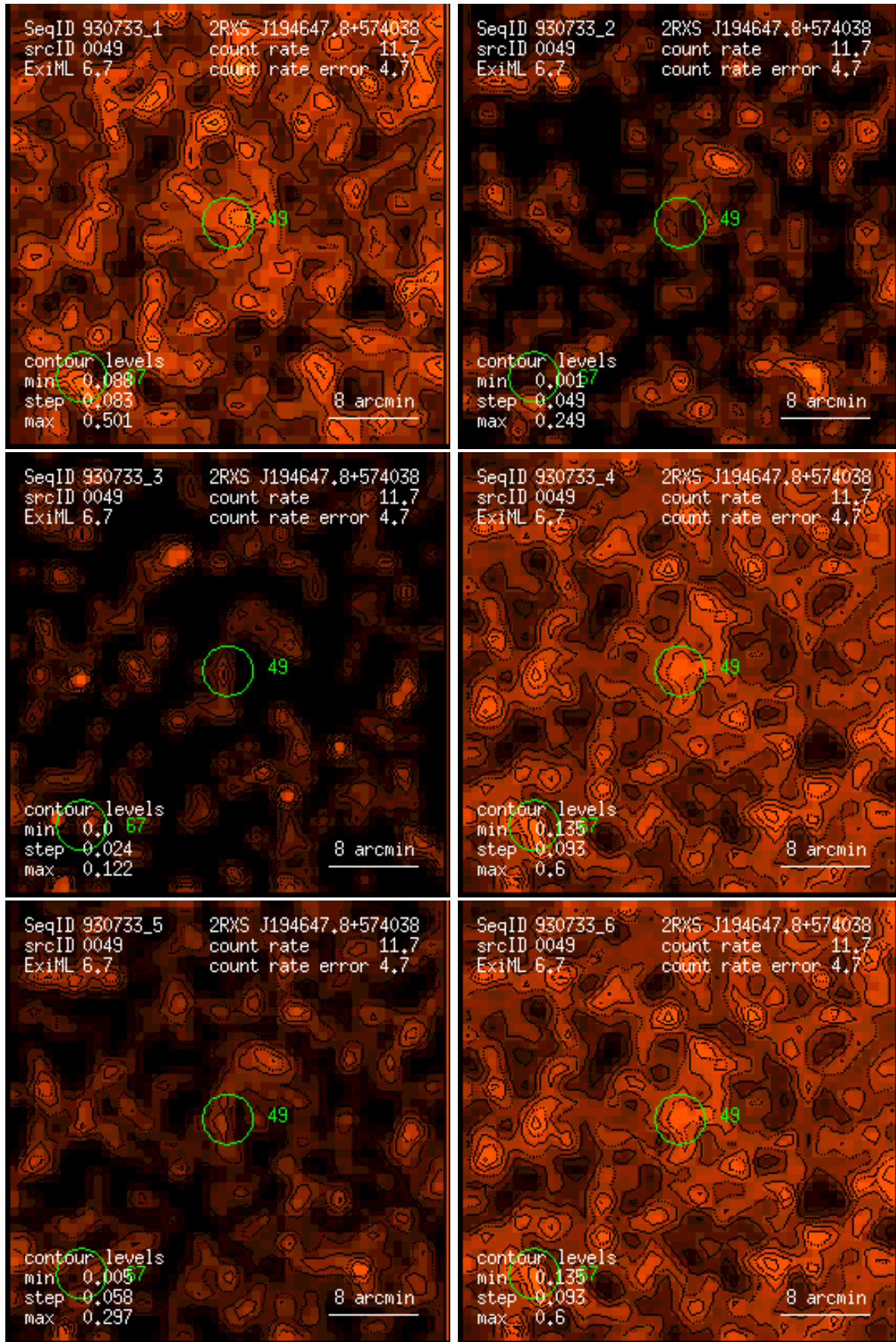
Figure 49: RASS 930733: detection 0049: band rate images, Gaussian filter: (1) PSPC channels 11 – 41, (2) 52 – 90, (3) 91 – 201, (4) 11 – 235, (5) 52 – 201, (6) 11 – 201. Broad band rates in counts/ks. Band rate contour levels in counts/ks/arcmin 2 .
