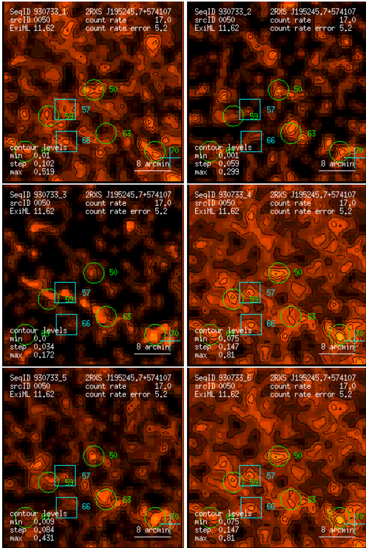
Figure 50: RASS 930733: detection 0050: band rate images, Gaussian filter: (1) PSPC channels 11 – 41, (2) 52 – 90, (3) 91 – 201, (4) 11 – 235, (5) 52 – 201, (6) 11 – 201. Broad band rates in counts/ks. Band rate contour levels in counts/ks/arcmin 2 .
