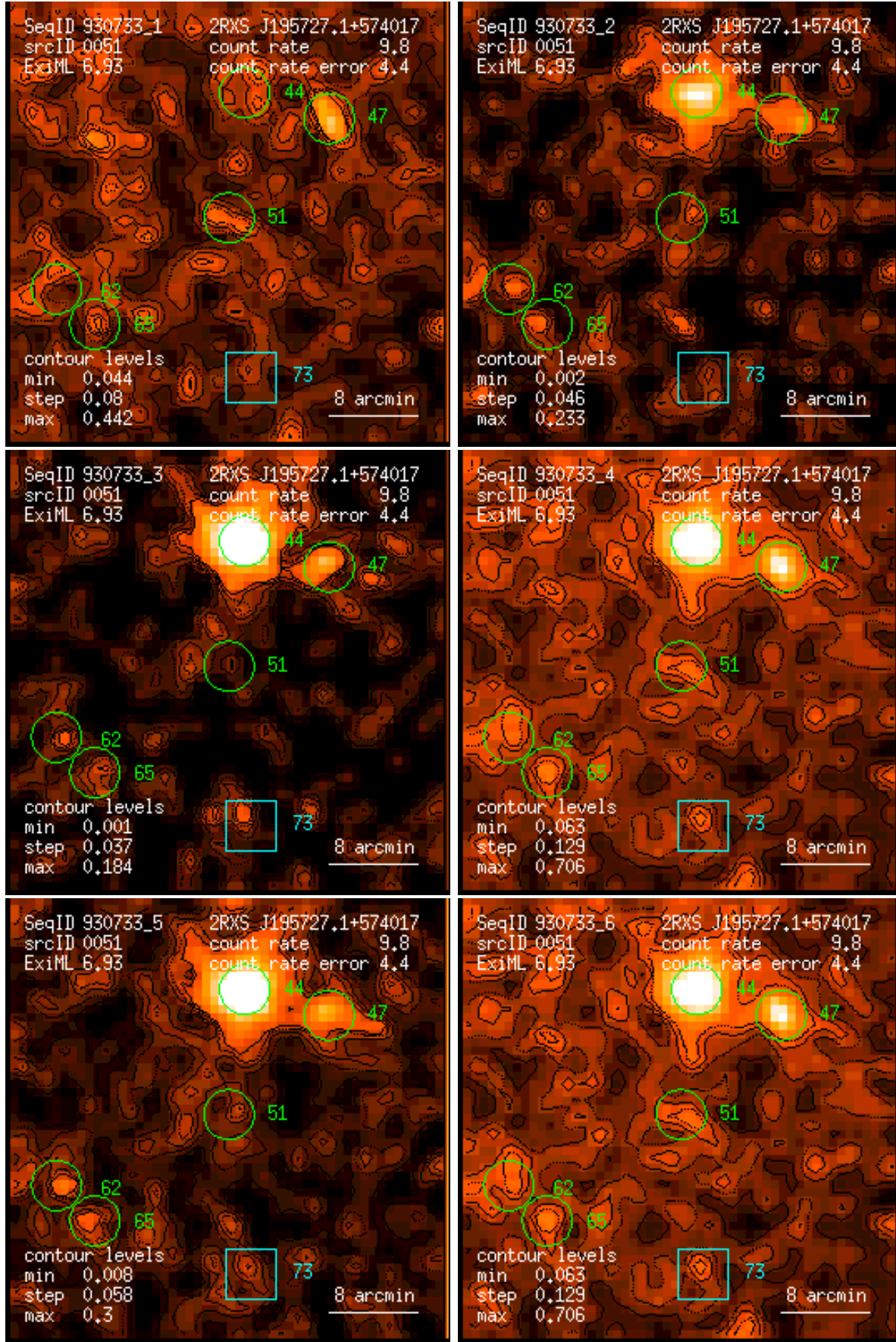
Figure 51: RASS 930733: detection 0051: band rate images, Gaussian filter: (1) PSPC channels 11 – 41, (2) 52 – 90, (3) 91 – 201, (4) 11 – 235, (5) 52 – 201, (6) 11 – 201. Broad band rates in counts/ks. Band rate contour levels in counts/ks/arcmin 2 .
