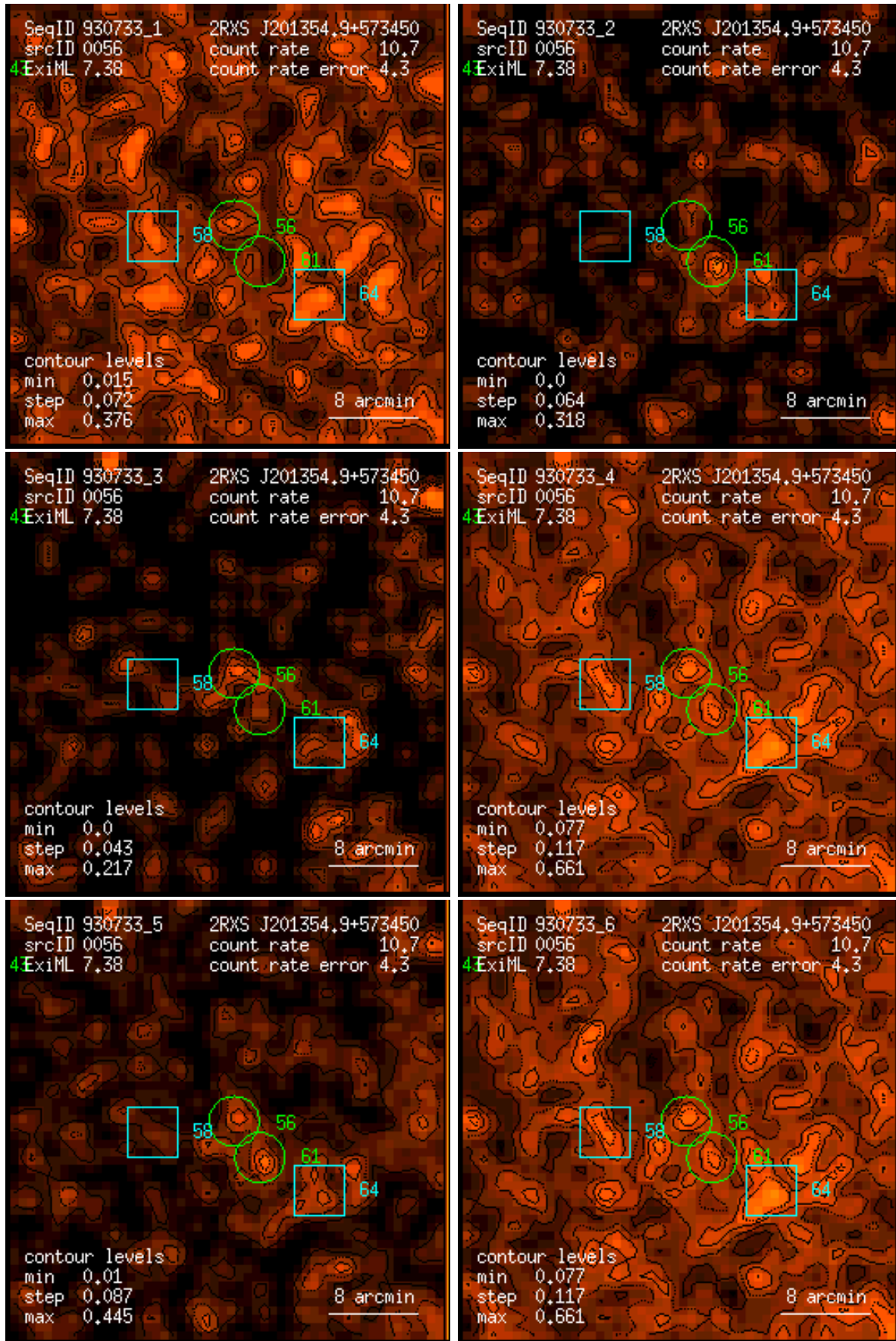
Figure 56: RASS 930733: detection 0056: band rate images, Gaussian filter: (1) PSPC channels 11 – 41, (2) 52 – 90, (3) 91 – 201, (4) 11 – 235, (5) 52 – 201, (6) 11 – 201. Broad band rates in counts/ks. Band rate contour levels in counts/ks/arcmin 2 .
