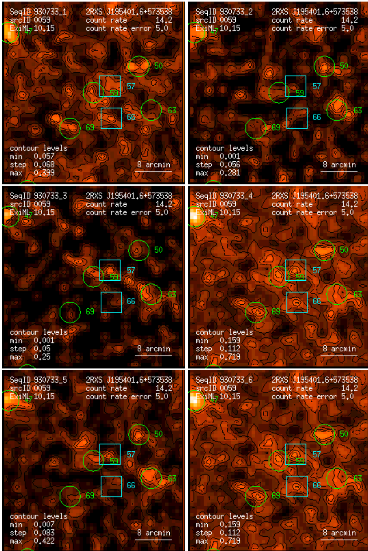
Figure 59: RASS 930733: detection 0059: band rate images, Gaussian filter: (1) PSPC channels 11 – 41, (2) 52 – 90, (3) 91 – 201, (4) 11 – 235, (5) 52 – 201, (6) 11 – 201. Broad band rates in counts/ks. Band rate contour levels in counts/ks/arcmin 2 .
