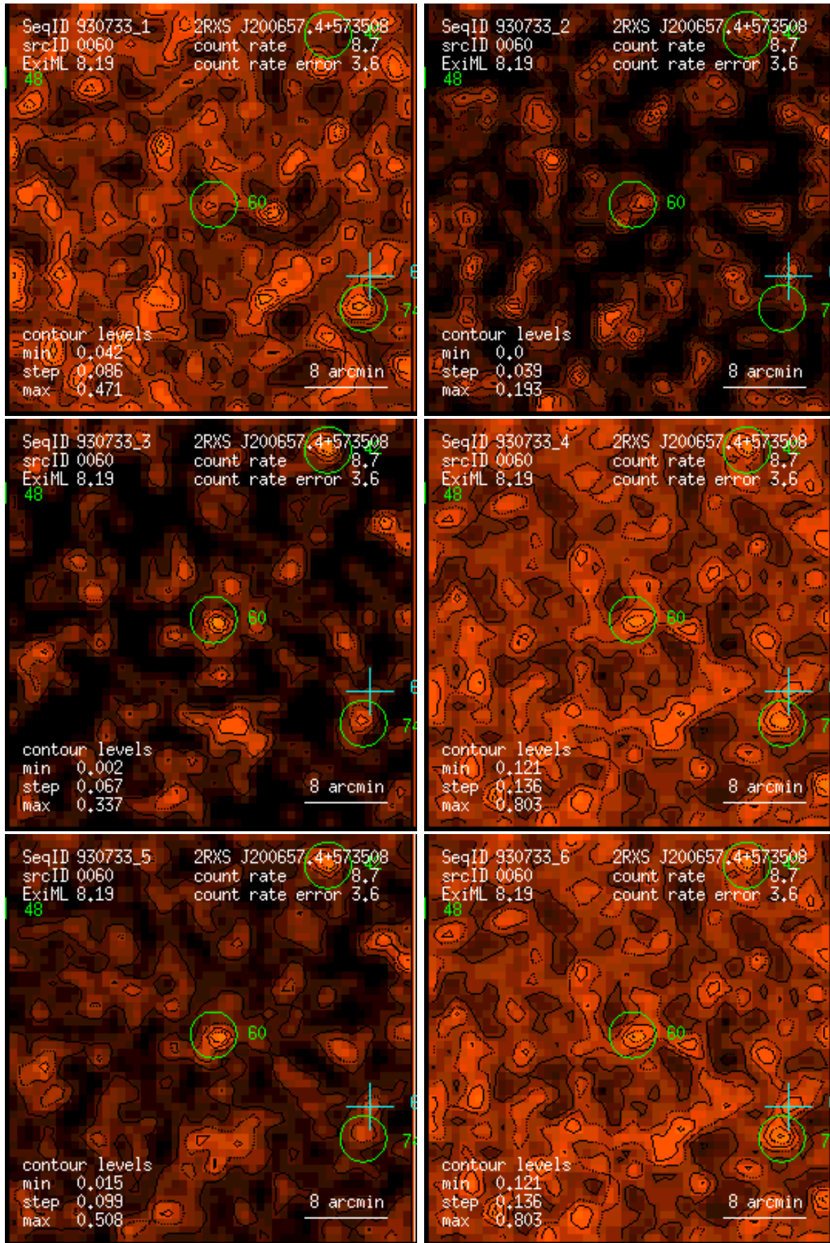
Figure 60: RASS 930733: detection 0060: band rate images, Gaussian filter: (1) PSPC channels 11 – 41, (2) 52 – 90, (3) 91 – 201, (4) 11 – 235, (5) 52 – 201, (6) 11 – 201. Broad band rates in counts/ks. Band rate contour levels in counts/ks/arcmin 2 .
