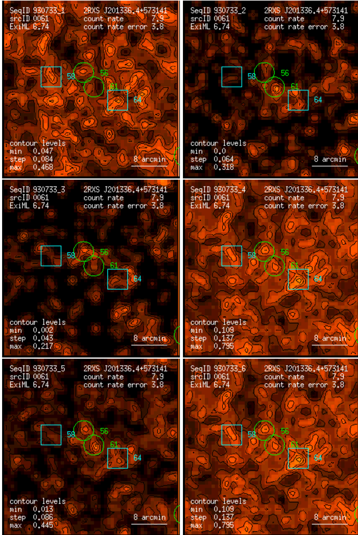
Figure 61: RASS 930733: detection 0061: band rate images, Gaussian filter: (1) PSPC channels 11 – 41, (2) 52 – 90, (3) 91 – 201, (4) 11 – 235, (5) 52 – 201, (6) 11 – 201. Broad band rates in counts/ks. Band rate contour levels in counts/ks/arcmin 2 .
