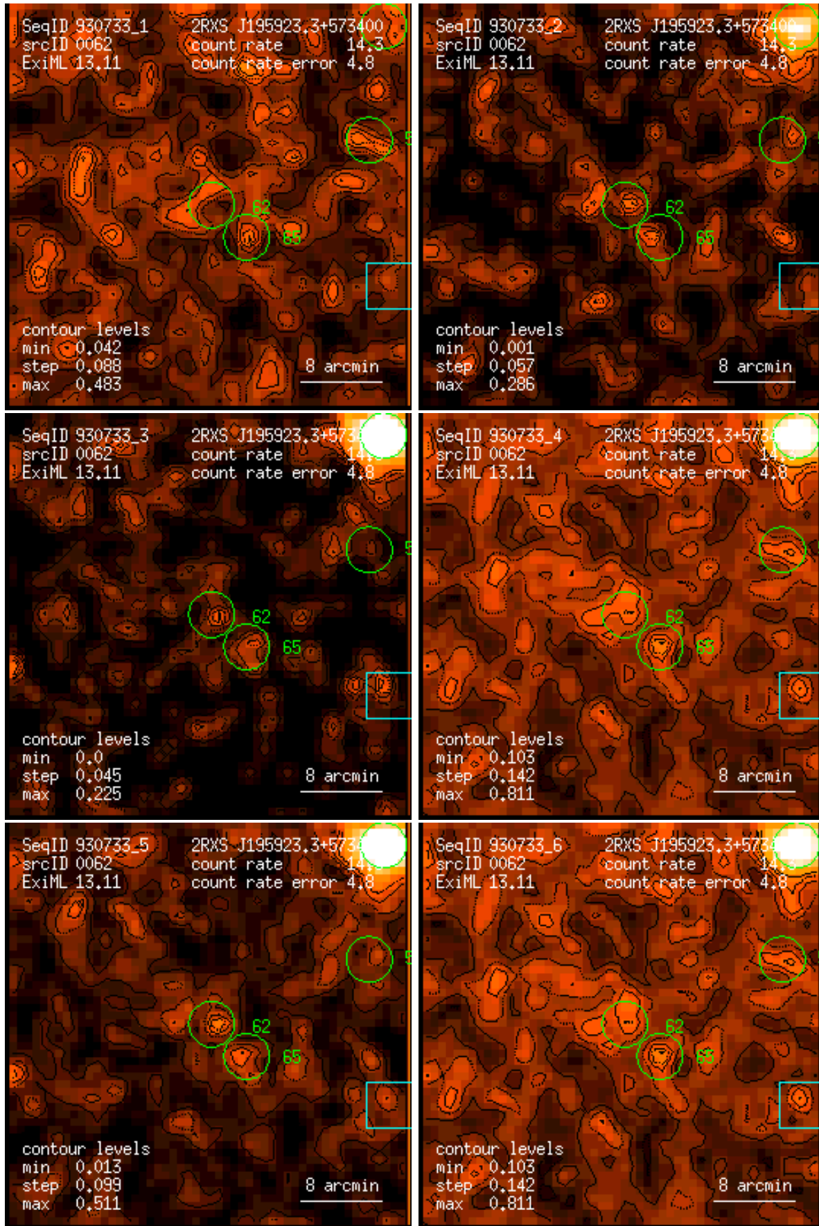
Figure 62: RASS 930733: detection 0062: band rate images, Gaussian filter: (1) PSPC channels 11 – 41, (2) 52 – 90, (3) 91 – 201, (4) 11 – 235, (5) 52 – 201, (6) 11 – 201. Broad band rates in counts/ks. Band rate contour levels in counts/ks/arcmin 2 .
