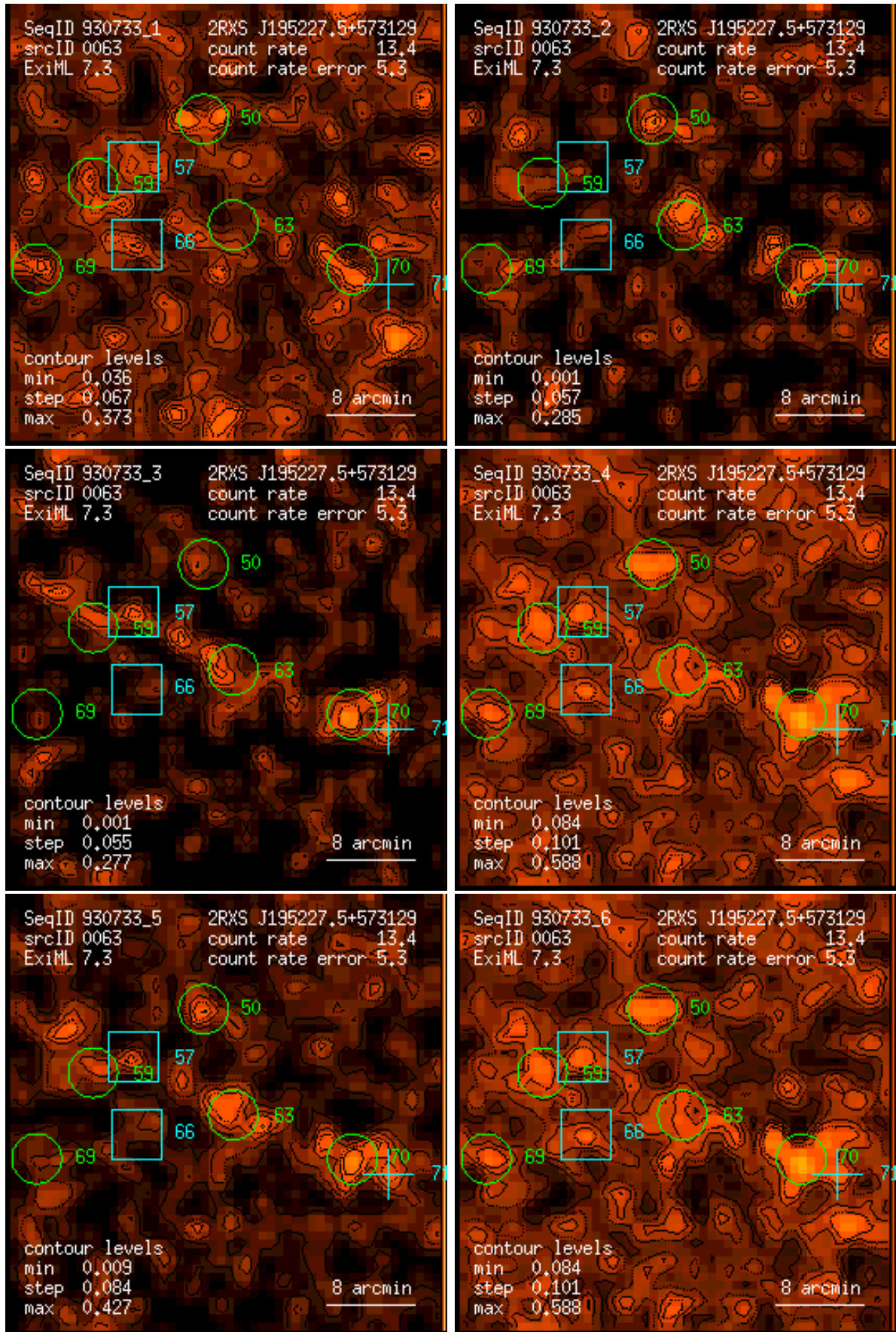
Figure 63: RASS 930733: detection 0063: band rate images, Gaussian filter: (1) PSPC channels 11 – 41, (2) 52 – 90, (3) 91 – 201, (4) 11 – 235, (5) 52 – 201, (6) 11 – 201. Broad band rates in counts/ks. Band rate contour levels in counts/ks/arcmin 2 .
