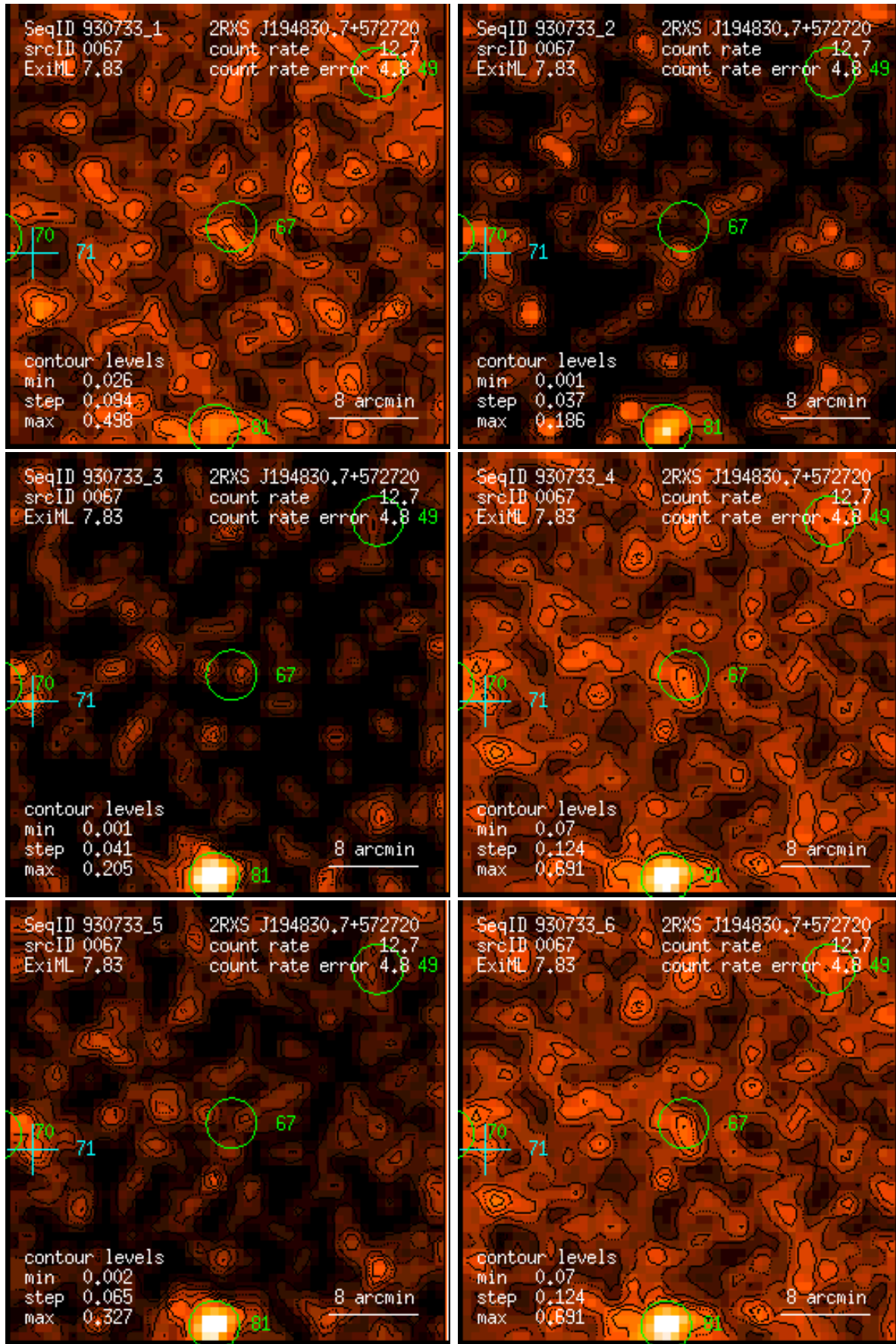
Figure 67: RASS 930733: detection 0067: band rate images, Gaussian filter: (1) PSPC channels 11 – 41, (2) 52 – 90, (3) 91 – 201, (4) 11 – 235, (5) 52 – 201, (6) 11 – 201. Broad band rates in counts/ks. Band rate contour levels in counts/ks/arcmin 2 .
