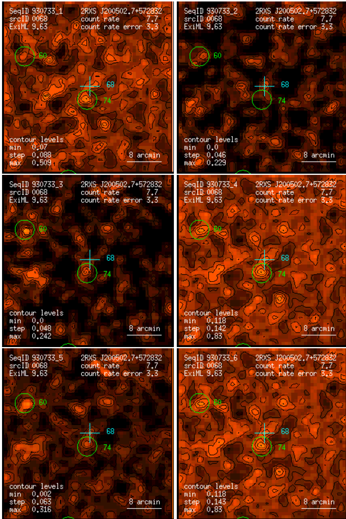
Figure 68: RASS 930733: detection 0068: band rate images, Gaussian filter: (1) PSPC channels 11 – 41, (2) 52 – 90, (3) 91 – 201, (4) 11 – 235, (5) 52 – 201, (6) 11 – 201. Broad band rates in counts/ks. Band rate contour levels in counts/ks/arcmin 2 .
