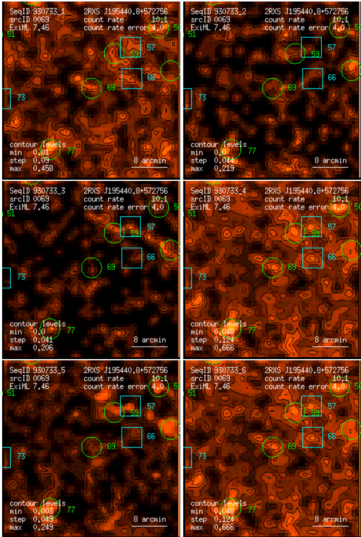
Figure 69: RASS 930733: detection 0069: band rate images, Gaussian filter: (1) PSPC channels 11 – 41, (2) 52 – 90, (3) 91 – 201, (4) 11 – 235, (5) 52 – 201, (6) 11 – 201. Broad band rates in counts/ks. Band rate contour levels in counts/ks/arcmin 2 .
