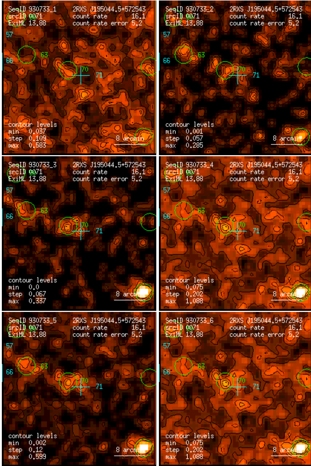
Figure 71: RASS 930733: detection 0071: band rate images, Gaussian filter: (1) PSPC channels 11 – 41, (2) 52 – 90, (3) 91 – 201, (4) 11 – 235, (5) 52 – 201, (6) 11 – 201. Broad band rates in counts/ks. Band rate contour levels in counts/ks/arcmin 2 .
