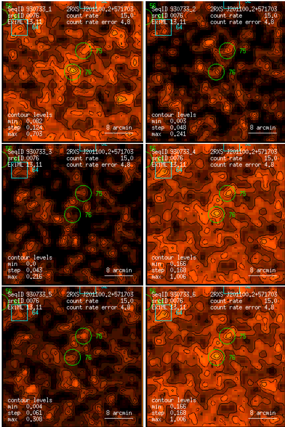
Figure 76: RASS 930733: detection 0076: band rate images, Gaussian filter: (1) PSPC channels 11 – 41, (2) 52 – 90, (3) 91 – 201, (4) 11 – 235, (5) 52 – 201, (6) 11 – 201. Broad band rates in counts/ks. Band rate contour levels in counts/ks/arcmin 2 .
