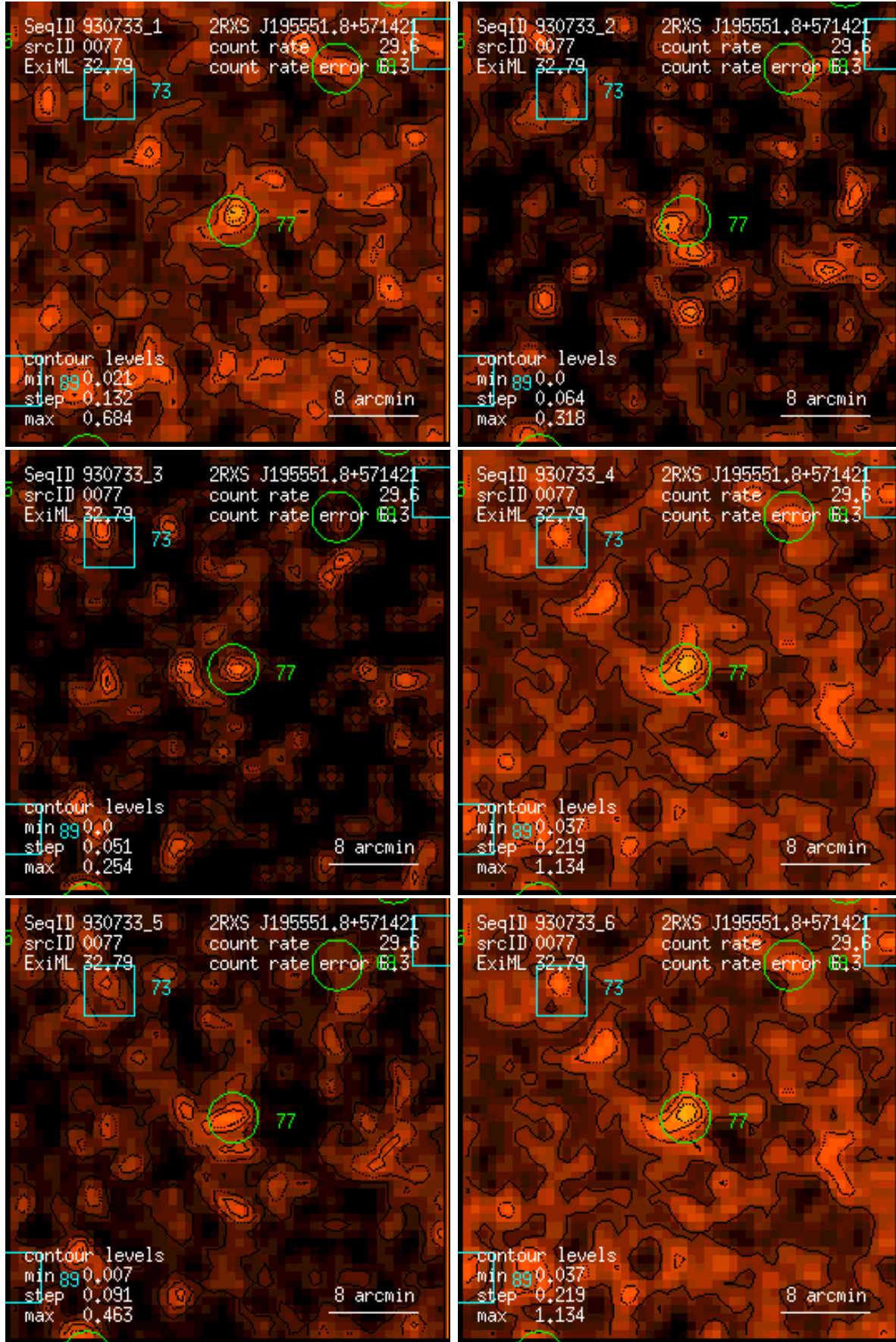
Figure 77: RASS 930733: detection 0077: band rate images, Gaussian filter: (1) PSPC channels 11 – 41, (2) 52 – 90, (3) 91 – 201, (4) 11 – 235, (5) 52 – 201, (6) 11 – 201. Broad band rates in counts/ks. Band rate contour levels in counts/ks/arcmin 2 .
