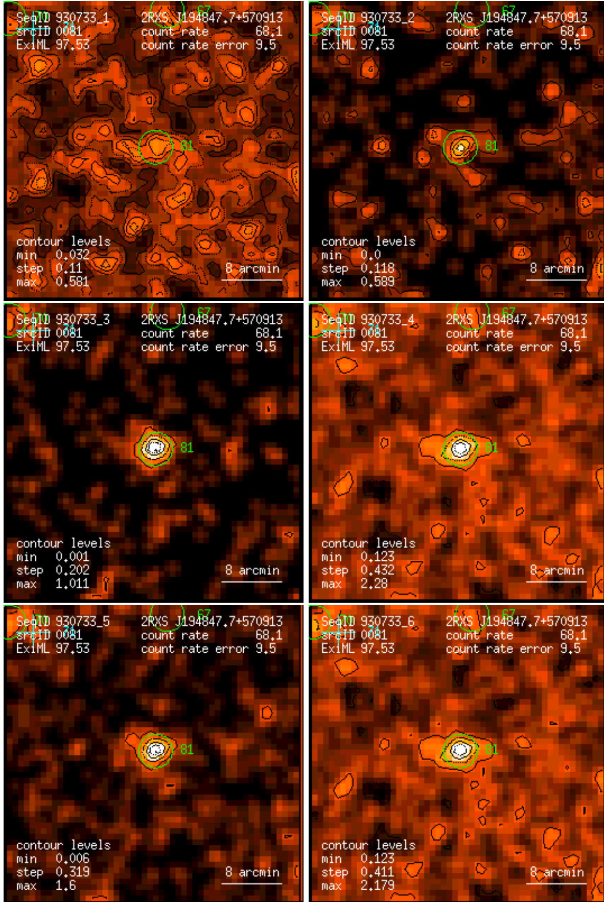
Figure 81: RASS 930733: detection 0081: band rate images, Gaussian filter: (1) PSPC channels 11 – 41, (2) 52 – 90, (3) 91 – 201, (4) 11 – 235, (5) 52 – 201, (6) 11 – 201. Broad band rates in counts/ks. Band rate contour levels in counts/ks/arcmin 2 .
