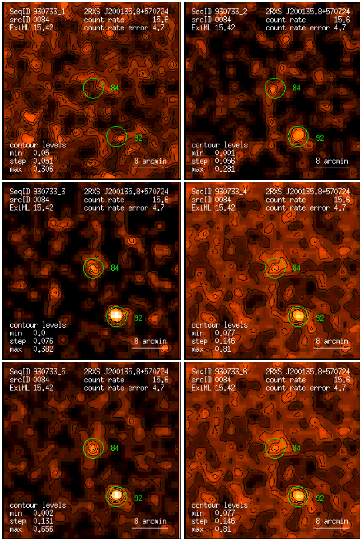
Figure 84: RASS 930733: detection 0084: band rate images, Gaussian filter: (1) PSPC channels 11 – 41, (2) 52 – 90, (3) 91 – 201, (4) 11 – 235, (5) 52 – 201, (6) 11 – 201. Broad band rates in counts/ks. Band rate contour levels in counts/ks/arcmin 2 .
