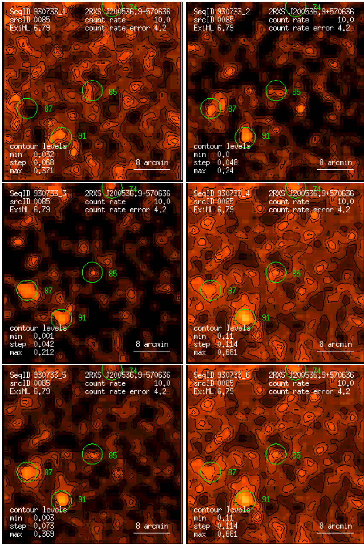
Figure 85: RASS 930733: detection 0085: band rate images, Gaussian filter: (1) PSPC channels 11 – 41, (2) 52 – 90, (3) 91 – 201, (4) 11 – 235, (5) 52 – 201, (6) 11 – 201. Broad band rates in counts/ks. Band rate contour levels in counts/ks/arcmin 2 .
