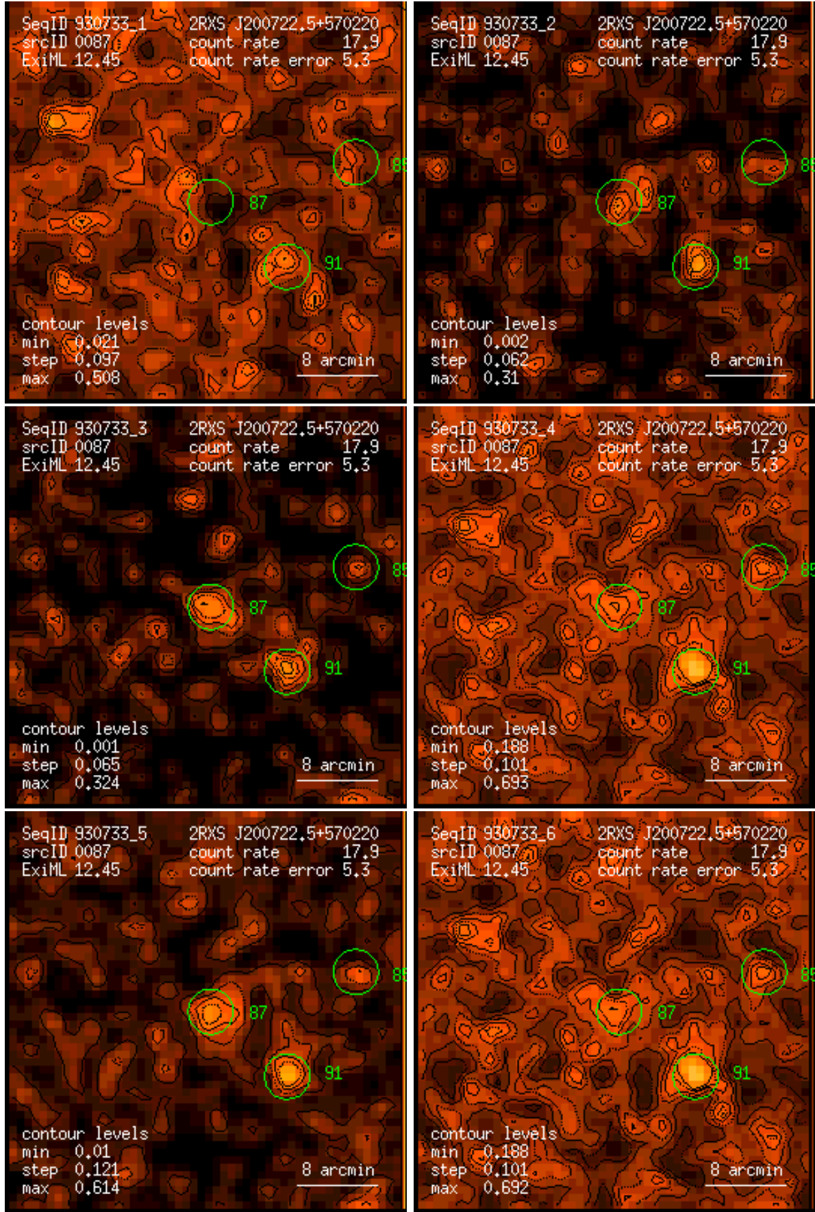
Figure 87: RASS 930733: detection 0087: band rate images, Gaussian filter: (1) PSPC channels 11 – 41, (2) 52 – 90, (3) 91 – 201, (4) 11 – 235, (5) 52 – 201, (6) 11 – 201. Broad band rates in counts/ks. Band rate contour levels in counts/ks/arcmin 2 .
