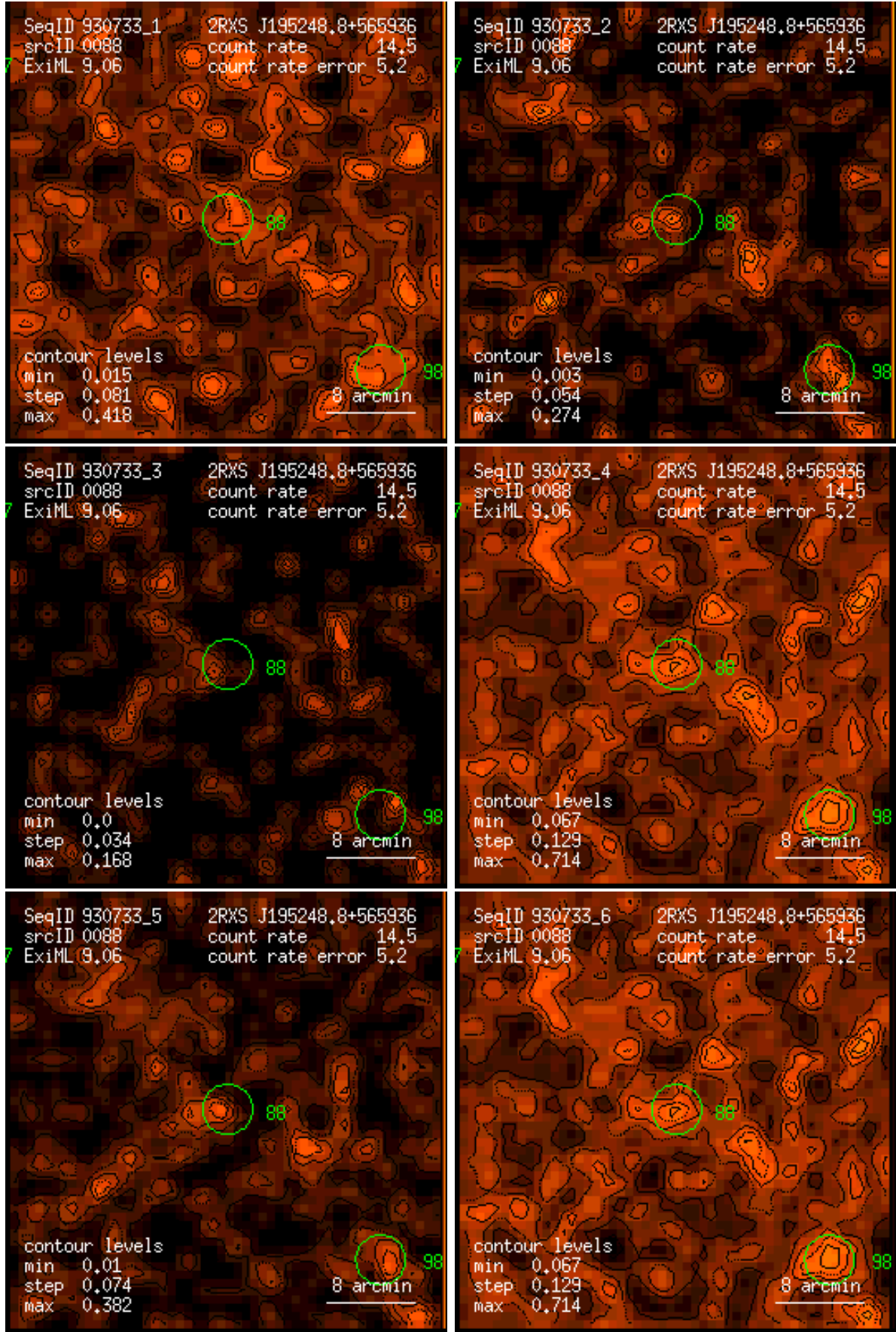
Figure 88: RASS 930733: detection 0088: band rate images, Gaussian filter: (1) PSPC channels 11 – 41, (2) 52 – 90, (3) 91 – 201, (4) 11 – 235, (5) 52 – 201, (6) 11 – 201. Broad band rates in counts/ks. Band rate contour levels in counts/ks/arcmin 2 .
