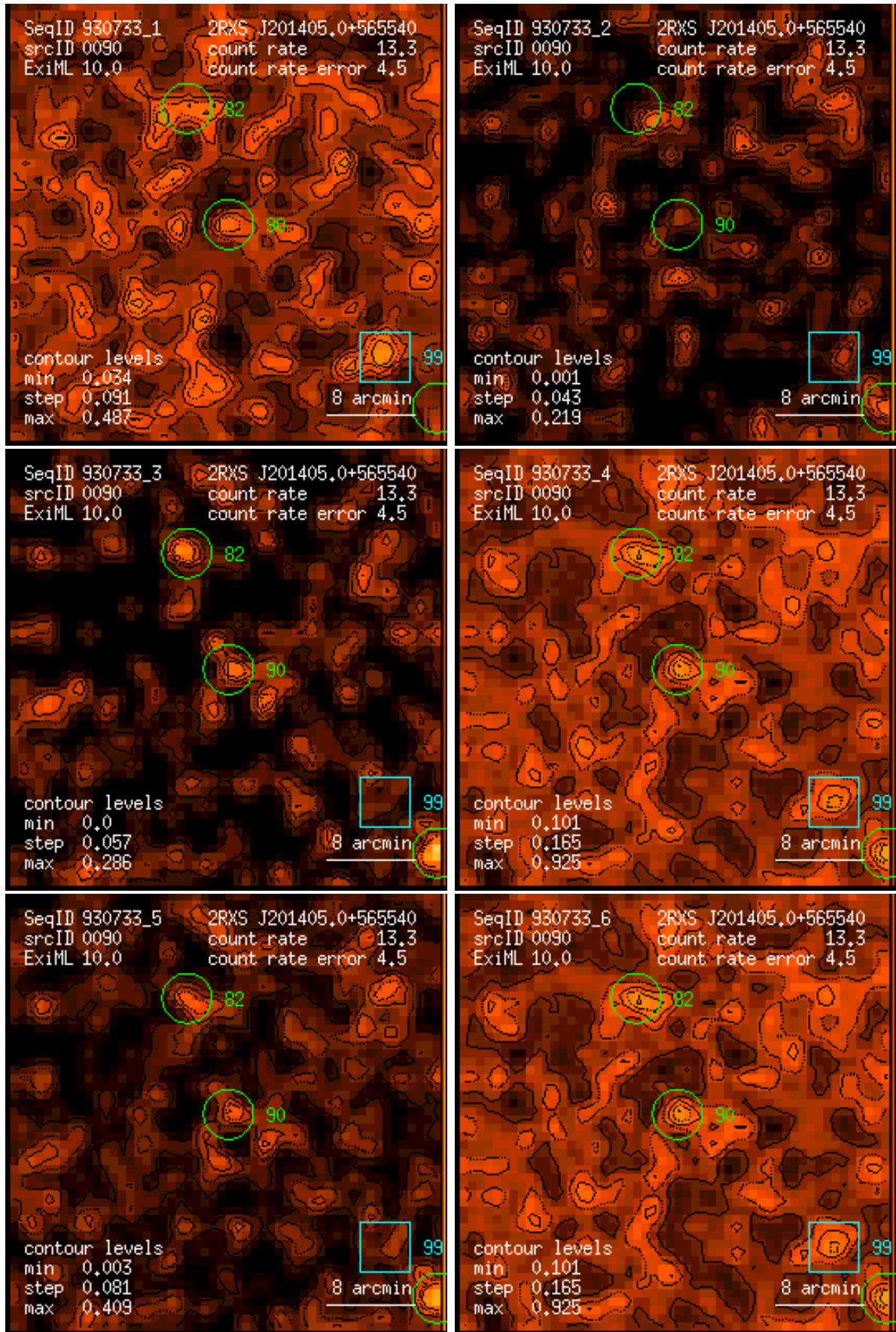
Figure 90: RASS 930733: detection 0090: band rate images, Gaussian filter: (1) PSPC channels 11 – 41, (2) 52 – 90, (3) 91 – 201, (4) 11 – 235, (5) 52 – 201, (6) 11 – 201. Broad band rates in counts/ks. Band rate contour levels in counts/ks/arcmin 2 .
