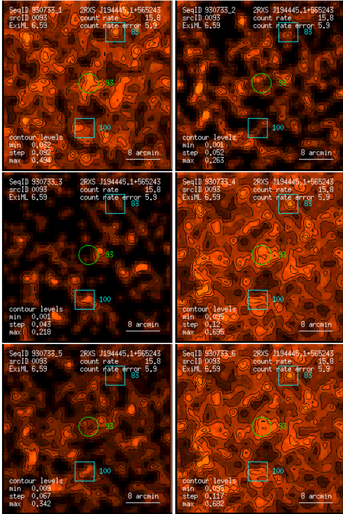
Figure 93: RASS 930733: detection 0093: band rate images, Gaussian filter: (1) PSPC channels 11 – 41, (2) 52 – 90, (3) 91 – 201, (4) 11 – 235, (5) 52 – 201, (6) 11 – 201. Broad band rates in counts/ks. Band rate contour levels in counts/ks/arcmin 2 .
