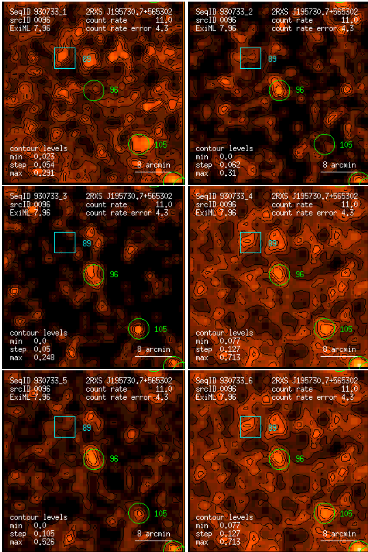
Figure 96: RASS 930733: detection 0096: band rate images, Gaussian filter: (1) PSPC channels 11 – 41, (2) 52 – 90, (3) 91 – 201, (4) 11 – 235, (5) 52 – 201, (6) 11 – 201. Broad band rates in counts/ks. Band rate contour levels in counts/ks/arcmin 2 .
