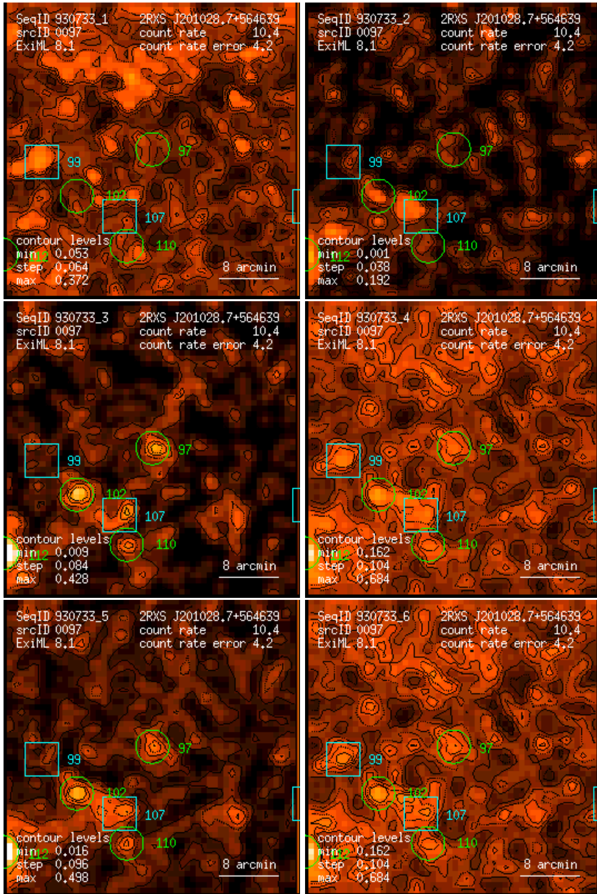
Figure 97: RASS 930733: detection 0097: band rate images, Gaussian filter: (1) PSPC channels 11 – 41, (2) 52 – 90, (3) 91 – 201, (4) 11 – 235, (5) 52 – 201, (6) 11 – 201. Broad band rates in counts/ks. Band rate contour levels in counts/ks/arcmin 2 .
