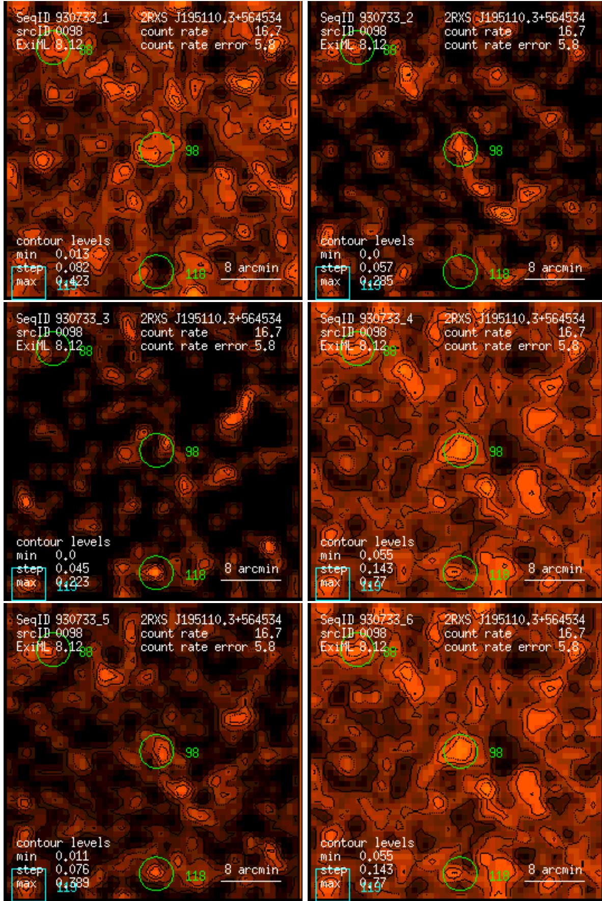
Figure 98: RASS 930733: detection 0098: band rate images, Gaussian filter: (1) PSPC channels 11 – 41, (2) 52 – 90, (3) 91 – 201, (4) 11 – 235, (5) 52 – 201, (6) 11 – 201. Broad band rates in counts/ks. Band rate contour levels in counts/ks/arcmin 2 .
