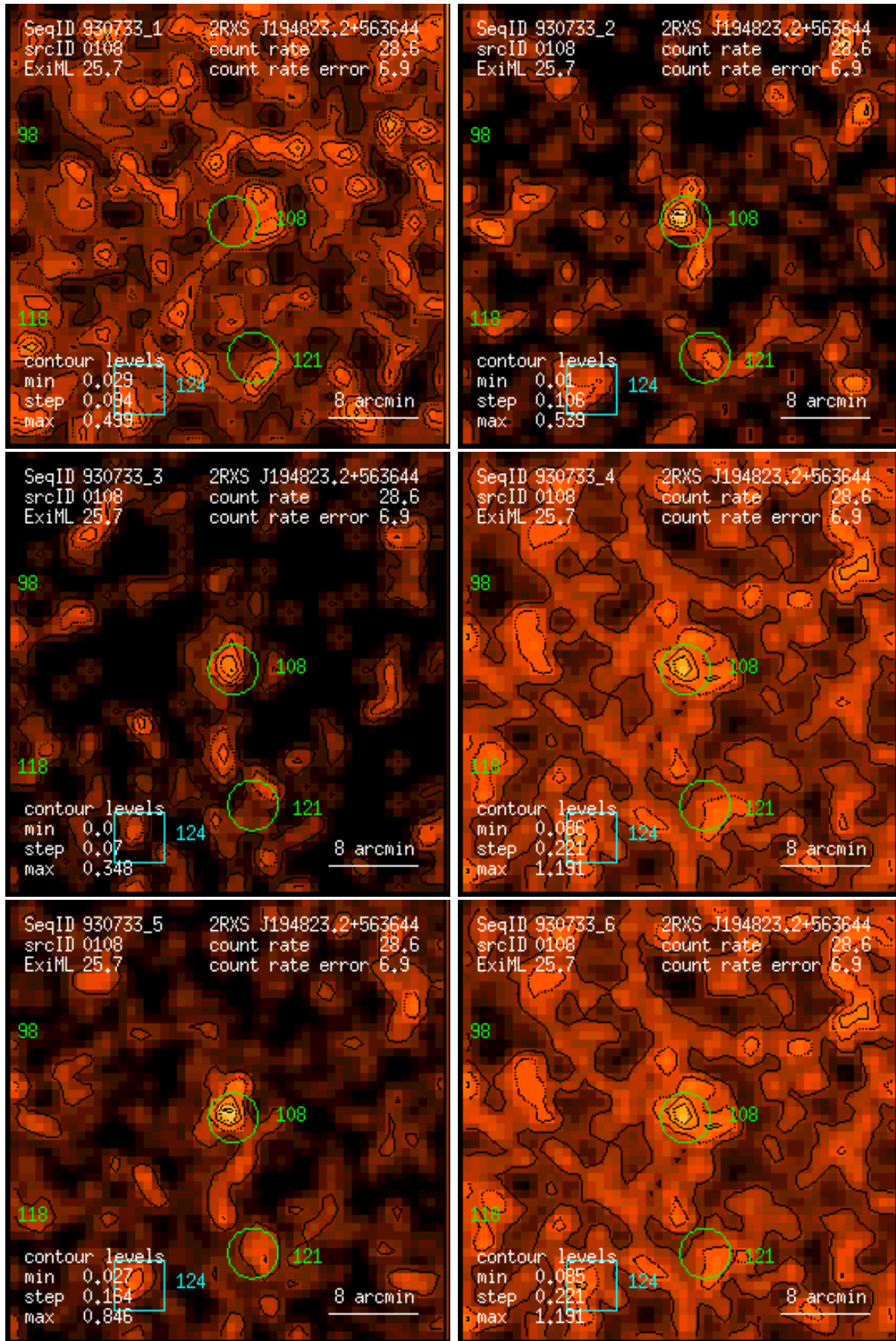
Figure 108: RASS 930733: detection 0108: band rate images, Gaussian filter: (1) PSPC channels 11 – 41, (2) 52 – 90, (3) 91 – 201, (4) 11 – 235, (5) 52 – 201, (6) 11 – 201. Broad band rates in counts/ks. Band rate contour levels in counts/ks/arcmin 2 .
