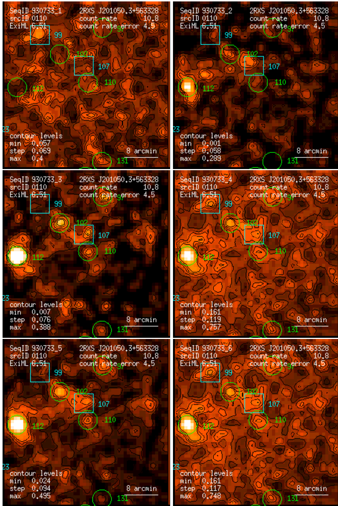
Figure 110: RASS 930733: detection 0110: band rate images, Gaussian filter: (1) PSPC channels 11 – 41, (2) 52 – 90, (3) 91 – 201, (4) 11 – 235, (5) 52 – 201, (6) 11 – 201. Broad band rates in counts/ks. Band rate contour levels in counts/ks/arcmin 2 .
